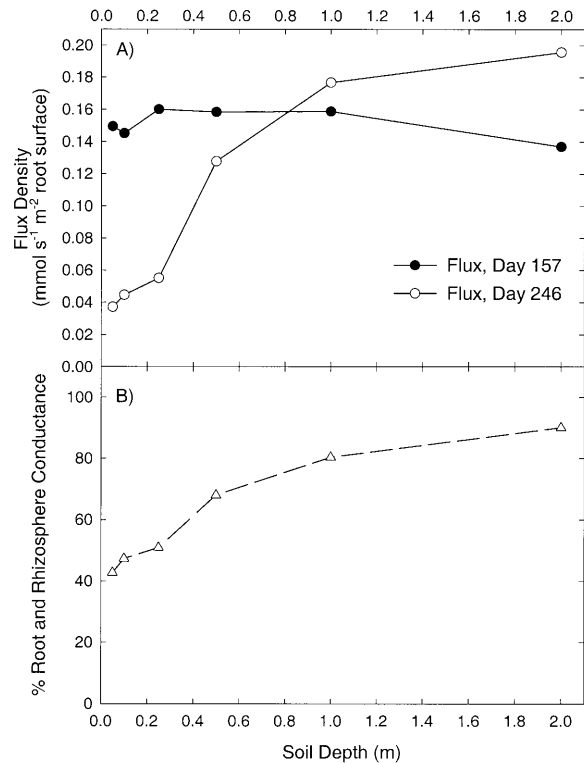
Fig. 8 A Flux density at the root surface for the six soil layers at the sand site (Fig. 1). Flux density is shown for first and last days of the 1997 data set (Fig. 4C), which represent maximum and minimum average \Psi_S over the period. B Hydraulic conductance at the sand site from bulk soil to root collar for each soil layer expressed as a percentage of the value on the first day. Data from the last day of the 1997 data set
