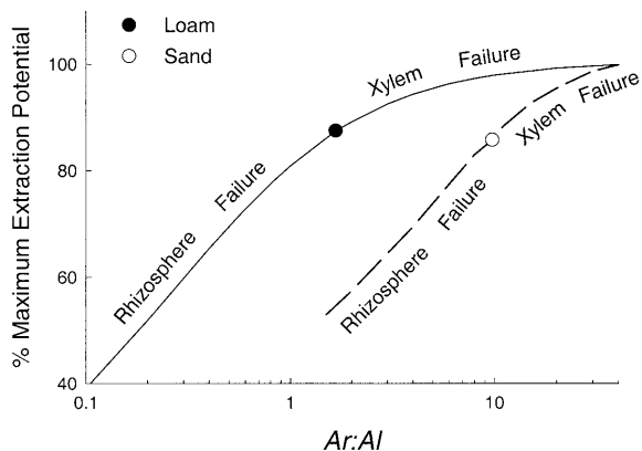
Fig. 7 Extraction potential vs A_R:A_L ( Ar:Al ) for loam (solid line) and sand (dashed line). Extraction potential is defined as area under the E_{crit} vs \Psi_S curve for the field range of \Psi_S (Fig. 6). Extraction potential is expressed as a percentage of the value at A_R:A_L=40 . This value was chosen as a liberal estimate of the maximum likely physiological value for a woody plant. Symbols correspond to measured values of A_R:A_L for loam (solid circle) and sand (open circle)
