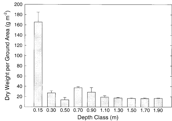
Fig. 3 Fine-root biomass vs depth at the sand site. Biomass means are shown with standard errors for n=4 soil pits. Fine roots were less than 1 mm in diameter. In contrast, 95% of fine roots at the loam site were in the top 0.2 m of soil (Matamala et al. 1998)
