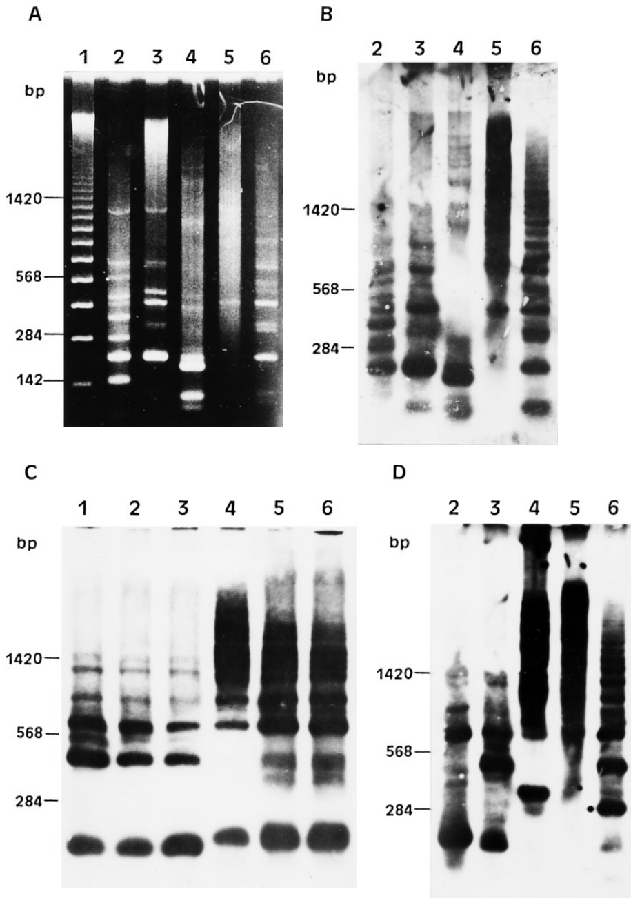
Fig. 1. A Electrophoretic separation of T. madens genomic DNA on 1.2% agarose gel; 5 \mu g of DNA was digested with AluI (lane 2), Clal (3), HinfI (4), Sau3A (5), and TaqI (6). T. molitor satellite DNA, partially digested with EcoRI , is used as a size marker (lane 1). B The Southern blot of gel shown in A after hybridization with cloned T.
