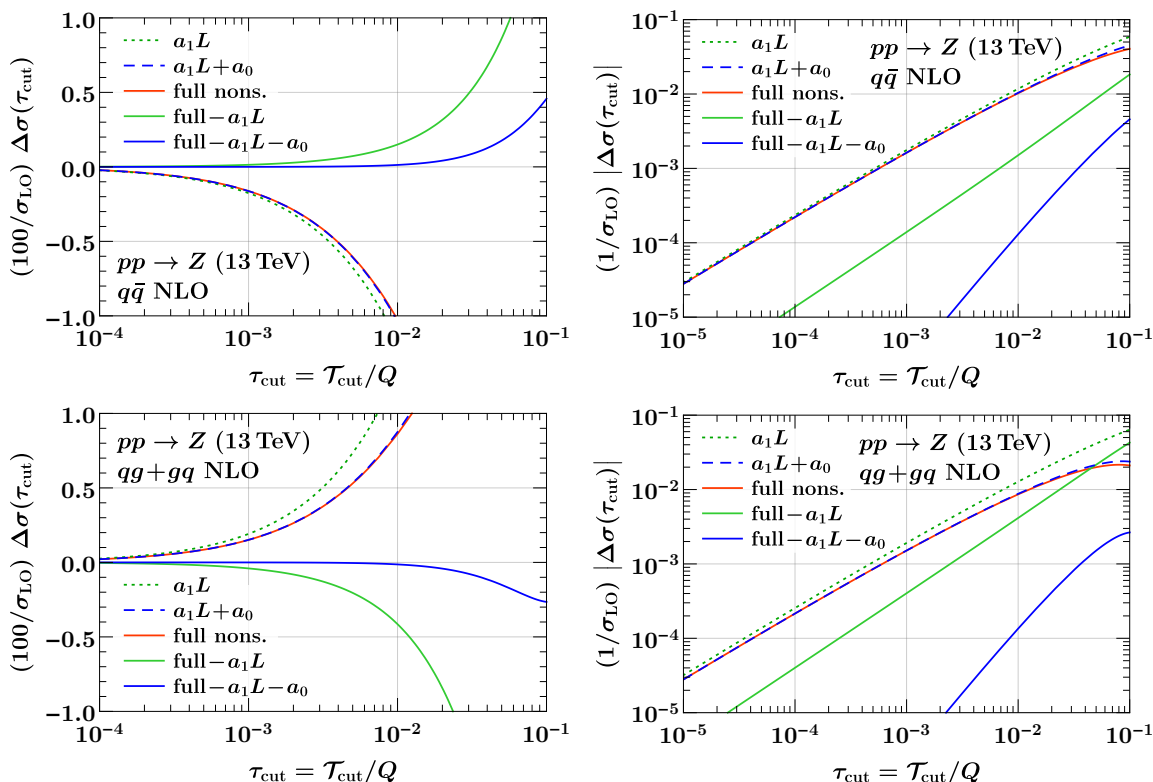
Figure 3. The power corrections for the cumulative \Delta\sigma(\tau_{\text{cut}}) at \mathcal{O}(\alpha_s) for Z production in the q\bar{q} channel (top row) and qg + gq channel (bottom row). In both cases, after the inclusion of the NLL power corrections, \Delta\sigma(\tau_{\text{cut}}) is reduced by a factor of 100 or more for \tau_{\text{cut}} < 10^{-2} .
