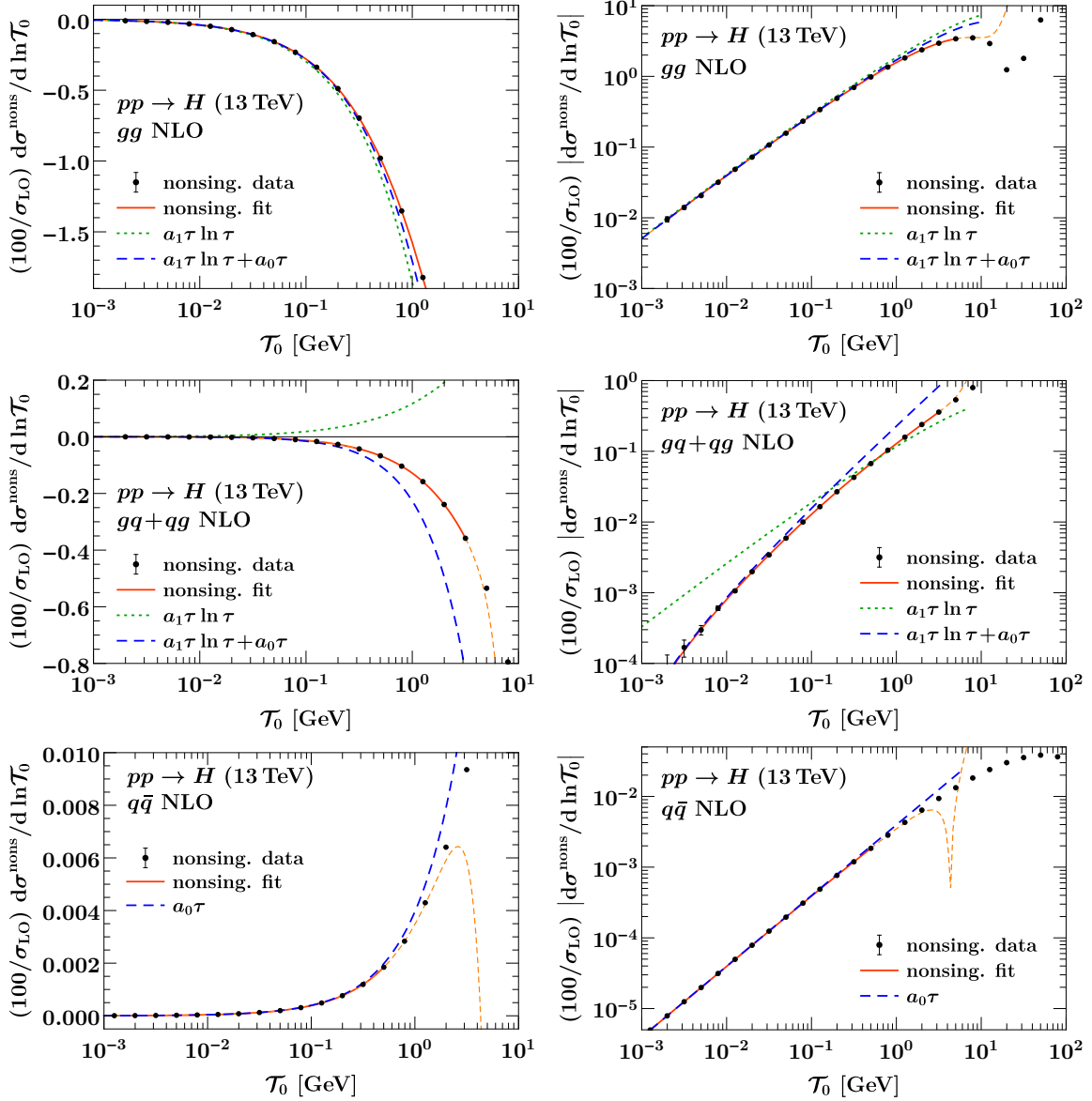
Figure 7. The \mathcal{O}(\alpha_s) nonsingular corrections for Higgs production for the gg channel (top row), gg+qg channel (middle row), and q\bar{q} channel (bottom row). A fit to the nonsingular data (black dots) is shown by the solid red curve. The LL and NLL results are shown by green dotted and blue dashed curves, respectively. In all cases, the NLL approximation provides an excellent approximation to the complete nonsingular cross section for sufficiently small \mathcal{T}_0 .
