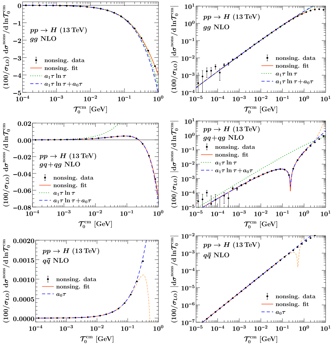
Figure 9. Same as figure 7 for the hadronic \mathcal{T} definition.
