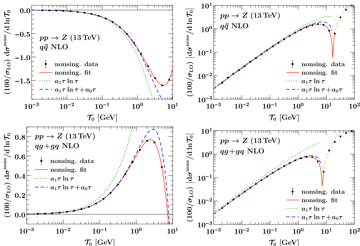
Figure 2. The \mathcal{O}(\alpha_s) nonsingular corrections for Z production for the q\bar{q} channel (top row) and the qg + gq channel (bottom row). A fit to the nonsingular data is shown by the solid red curve. The LL and NLL results are shown by green dotted and blue dashed curves, respectively. In all cases, the NLL approximation provides an excellent approximation to the complete nonsingular cross section.
