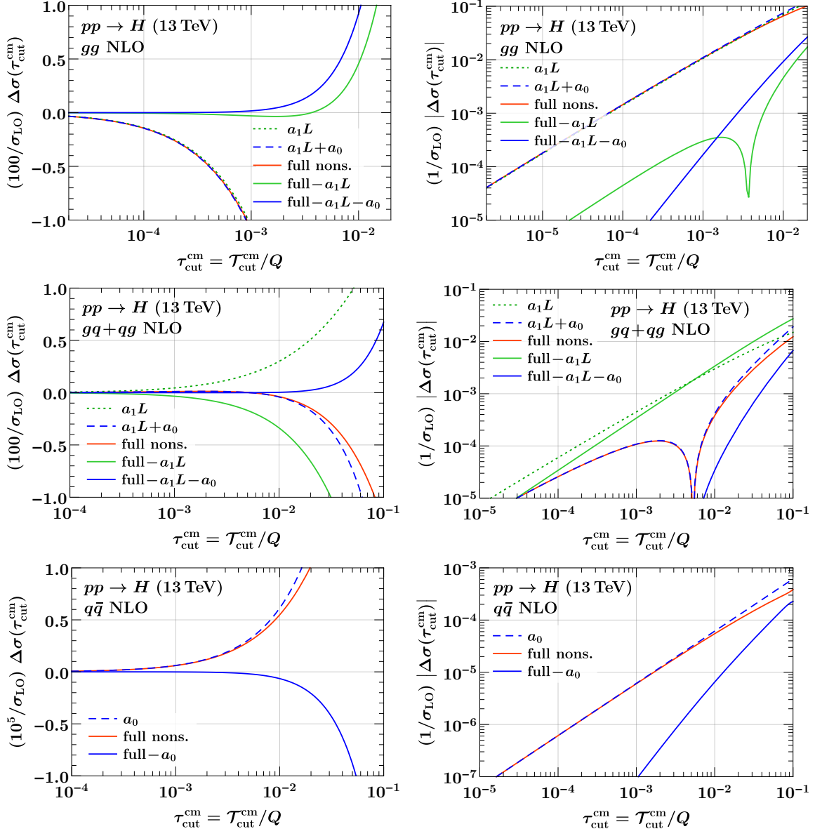
Figure 10. Same as figure 8 for the hadronic \mathcal{T} definition.
