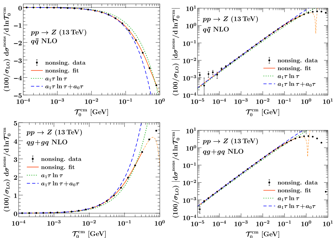
Figure 4. Same as figure 2 for the hadronic \mathcal{T} definition.
