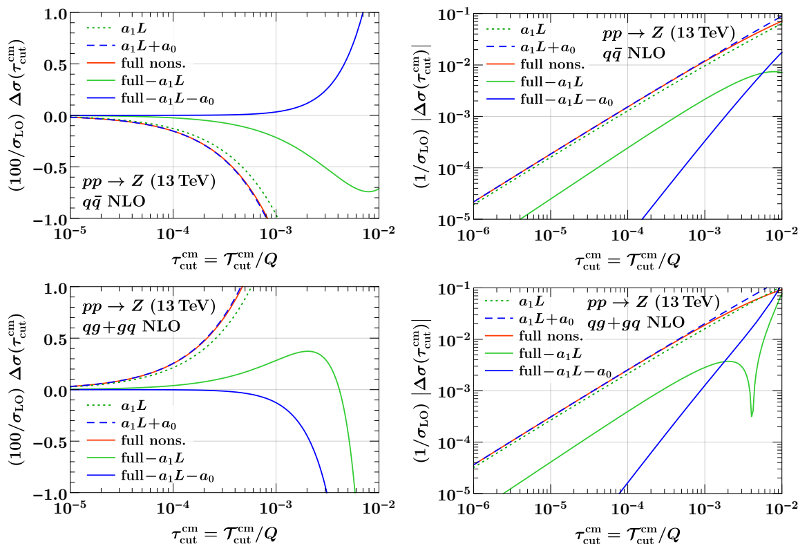
Figure 5. Same as figure 3 for the hadronic \mathcal{T} definition.
