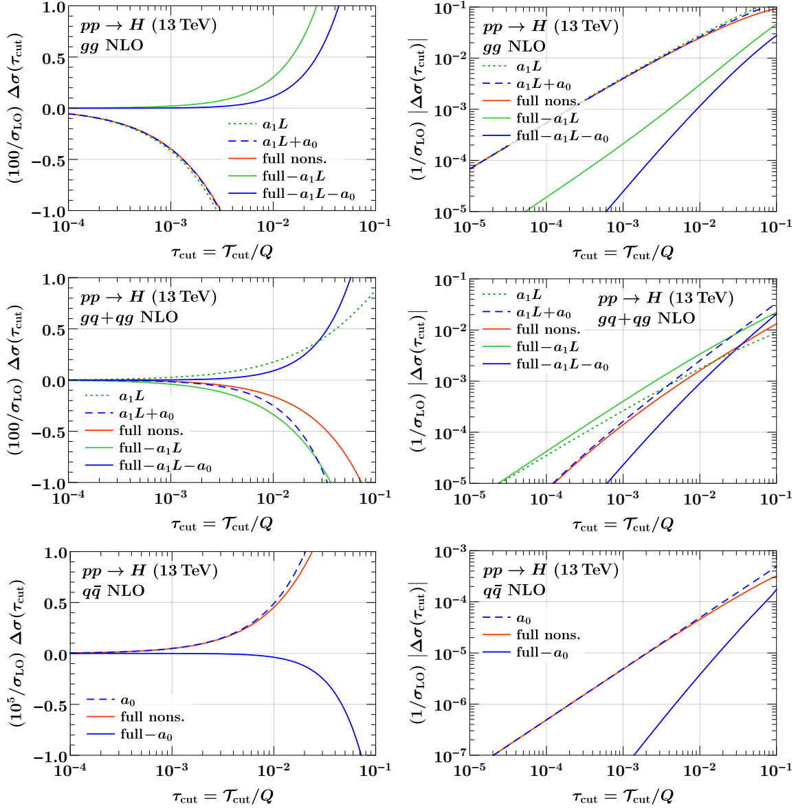
Figure 8. The power corrections for the cumulant \Delta\sigma(\tau_{\text{cut}}) at \mathcal{O}(\alpha_s) for Higgs production in the gg channel (top row), gq + qg channel (middle row), q\bar{q} channel (bottom row).
