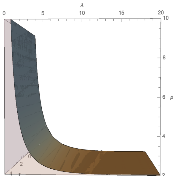
Figure 6. Schematic plot of the critical surface. The gray region represents the weak coupling phase.
