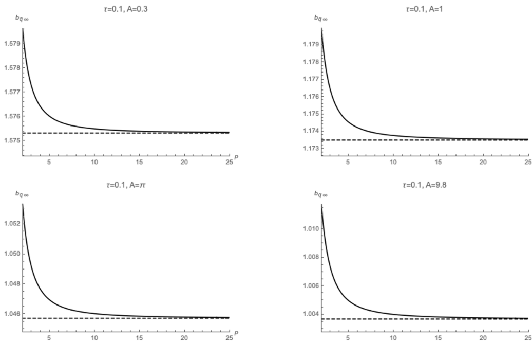
Figure 8. Plot of b_{q,\infty} as a function of p at \tau = 0.1 . The four plots correspond to A = 0.3, 1, \pi, 9.8 . The dashed horizontal line is the corresponding value of b_\infty in T\bar{T} -deformed Yang-Mills theory without q -deformation.
