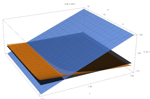
Figure 11. Plot of b_{q,\infty} as a function of p , at A = 1 and \tau = 0.1 . The blue surface is the function x on the left-hand side of (A.1). The orange surface is the right-hand side of (A.1) as a function of p and x . b_{q,\infty} is determined by the intersection of these two surfaces. The black horizontal surface is the asymptotic value b_\infty .
