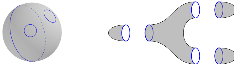
Figure 3. A sphere with three Wilson loops is cut into three disks plus a remaining pair of pants.
