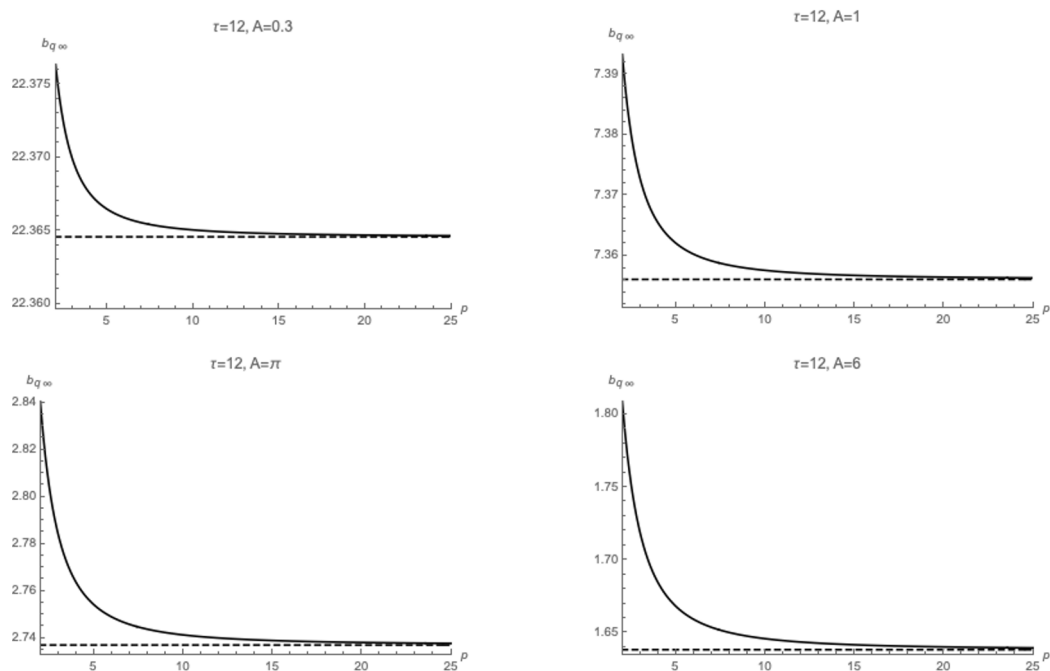
Figure 10. Plot of b_{q,\infty} as a function of p at \tau = 12 . The four plots correspond to A = 0.3, 1, \pi, 6 . The dashed horizontal line is the corresponding value of b_\infty in T\bar{T} -deformed Yang-Mills theory without q -deformation.
