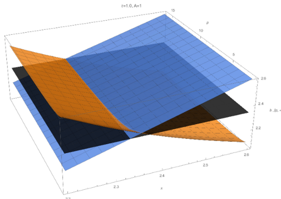
Figure 12. Plot of b_{q,\infty} as a function of p , at A = 1 and \tau = 1.0 . The blue surface is the function x on the left-hand side of (A.1). The orange surface is the right-hand side of (A.1) as a function of p and x . b_{q,\infty} is determined by the intersection of these two surfaces. The black horizontal surface is the asymptotic value b_\infty .
