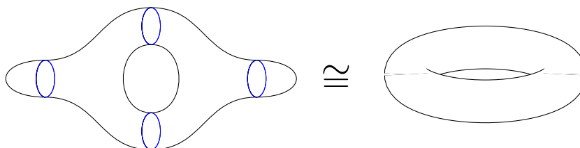
Figure 2. Obtaining a torus from elementary pieces. On the left, the gluing is an integration over boundary conditions (in blue).
