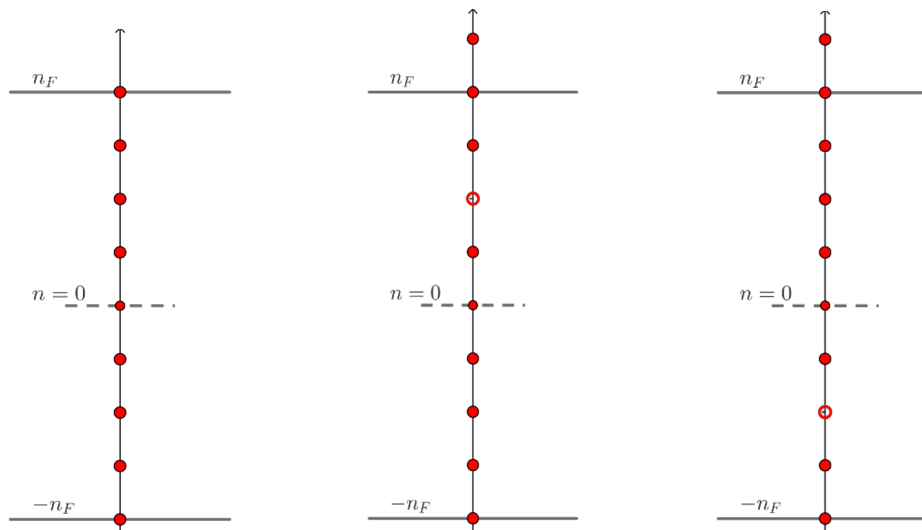
Figure 4. Non-relativistic fermions: ground state (left) and two excited states (center, right). The two excited states are excitations over the positive Fermi surface. In the center, a fermion occupying a positive energy level jumps above the positive Fermi surface: this will correspond to a chiral state at large N . On the right, a fermion occupying a negative energy level jumps above the positive Fermi surface: this will be exponentially suppressed at large N .
