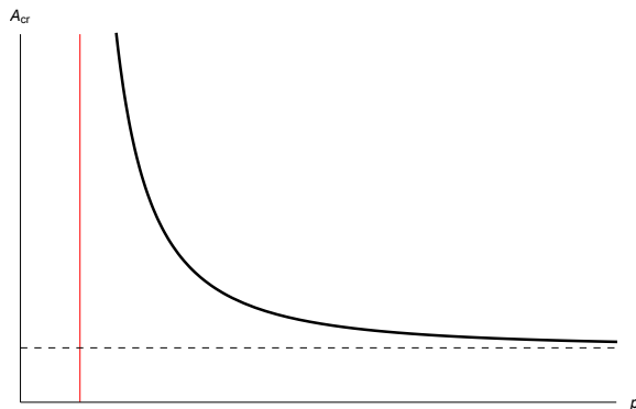
Figure 5. The critical curve of q -Yang-Mills theory, in terms of the parameter A = \lambda/p as a function of p . The horizontal asymptote (dashed) is the DK critical point A_{\text{cr}} = \pi^2 . The vertical asymptote (red) is the point p = 2 . This plot is inspired by [69].
