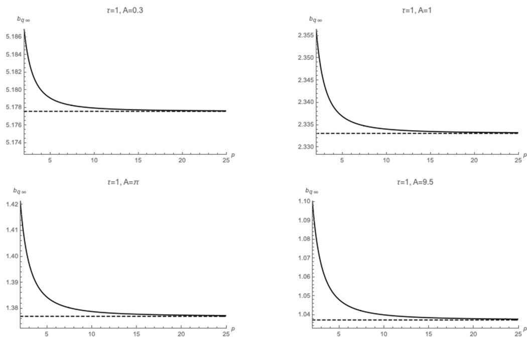
Figure 9. Plot of b_{q,\infty} as a function of p at \tau = 1 . The four plots correspond to A = 0.3, 1, \pi, 9.5 . The dashed horizontal line is the corresponding value of b_\infty in T\bar{T} -deformed Yang-Mills theory without q -deformation.
