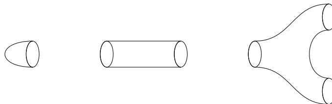
Figure 1. The disk (left), the cylinder (center) and the pair of pants (right), homeomorphic to the complex plane with respectively zero, one or two holes.
