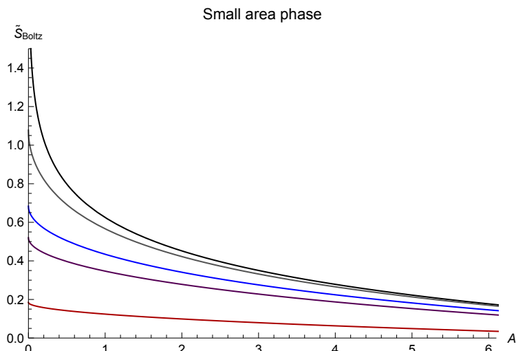
Figure 7. Entanglement entropy of T\bar{T} -deformed Yang-Mills theory at large N , normalized by N^2 and per number of entangling points, as a function of the area A in the weak coupling phase. The different curves correspond to the values \tau = 0 (black), \tau = 0.1 (gray), \tau = 0.5 (blue), \tau = 1 (purple), and \tau = 5 (red).
