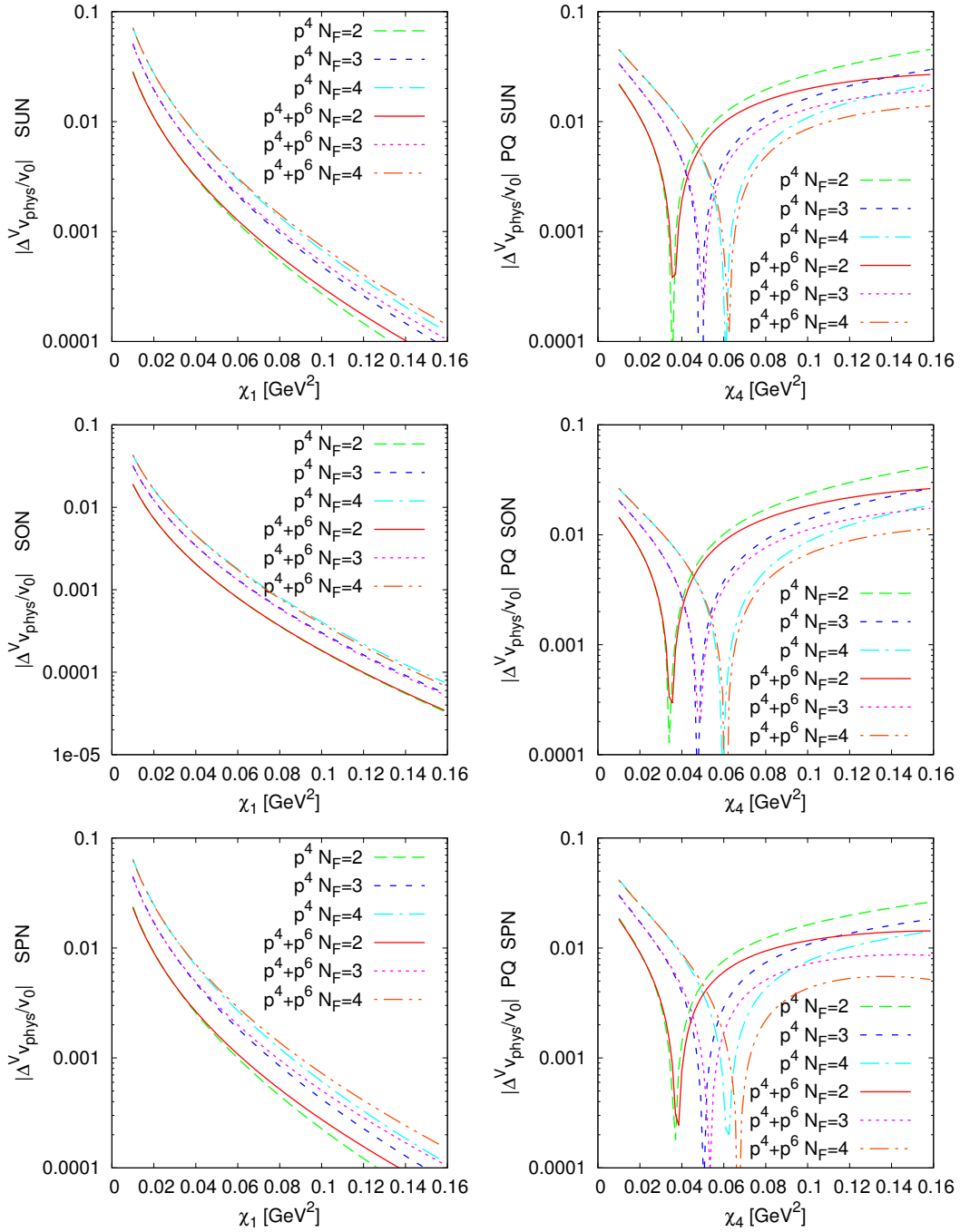
Figure 6. The absolute value of the finite volume correction to the vacuum expectation value divided by the lowest order value v_0 = v_{\text{LO}} for the unquenched (left) as a function of \chi_1 and the partially quenched case (right) as a function of \chi_4 with \chi_1 = 0.14^2 \text{ GeV}^2 . Shown are the NLO ( p^4 ) and NNLO ( p^4 + p^6 ) results for three values of N_F . Top line: SU(N_F) \times SU(N_F) \rightarrow SU(N_F) . Middle line: SU(N_F) \rightarrow SO(N_F) . Bottom line: SU(2N_F) \rightarrow \text{Sp}(2N_F) .
