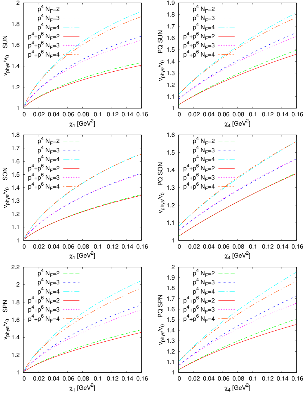
Figure 3. The vacuum expectation value divided by the lowest order value v_0 = v_{\text{LO}} for the unquenched (left) as a function of \chi_1 and the partially quenched case (right) as a function of \chi_4 with \chi_1 = 0.14^2 \text{ GeV}^2 . Other input as in the text. Shown are the NLO ( p^4 ) and NNLO ( p^4 + p^6 ) results for three values of N_F . Top line: SU(N_F) \times SU(N_F) \rightarrow SU(N_F) . Middle line: SU(N_F) \rightarrow SO(N_F) . Bottom line: SU(2N_F) \rightarrow \text{Sp}(2N_F) .
