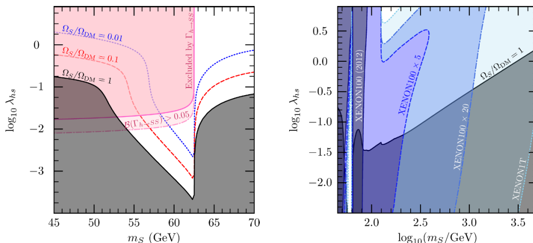
Figure 1. DM exclusion contours from ref. [59] on the \lambda_{hs} , m_s plane. Left plot is a close-up on the region m_s \lesssim m_h/2 . The dark-shaded lower region is ruled out by the upper bound on the singlet DM relic density, \Omega_S/\Omega_{DM} \leq 1 . The region in the upper-left corner is ruled out by constraints on invisible Higgs decays. Right plot is over a wide mass range 45 \text{ GeV} \leq m_s \leq 5 \text{ TeV} . The DM relic density exclusion is shown superimposed with the current bound from XENON100 and bounds from future direct detection experiments (in lighter shades of blue).
