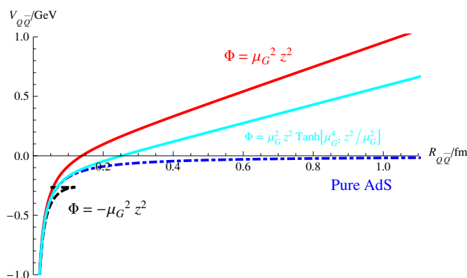
Figure 8. The quenched quark potential result V_{Q\bar{Q}} as functions of R_{Q\bar{Q}} in the quenched dynamical soft-wall model for the dilaton field \Phi = \mu_G^2 z^2 (red solid line), \Phi = -\mu_G^2 z^2 (black dashed line), \Phi = \mu_G^2 z^2 \tanh(\mu_G^4 z^2 / \mu_G^2) (cyan solid line), respectively. The blue dash-dotted line stands for the pure AdS 5 case. \mu_G = 1\text{GeV} and g_p = 0.4 have been used for numerical calculations.
