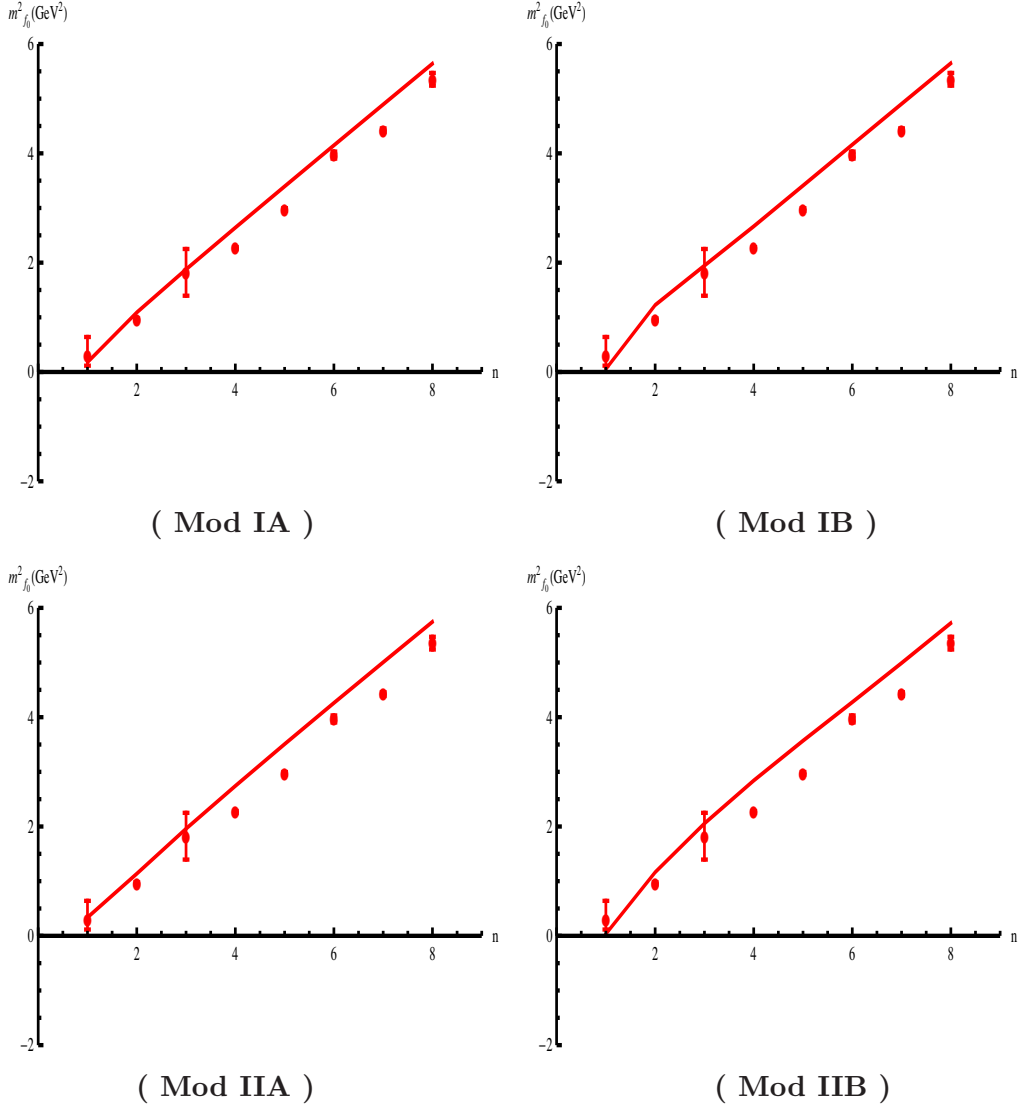
Figure 14. Scalar meson spectra m_{f_0, n}^2 as functions of n for Mod I and II defined in table 7.
