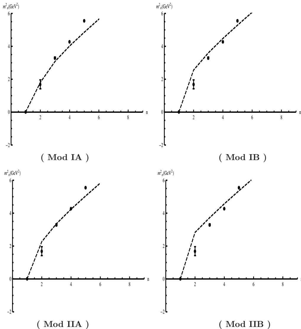
Figure 16. Pseudo-scalar spectra m_{\pi,n}^2 as functions of n for Mod I and II defined in table 7.
