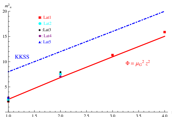
Figure 2. The 0 ++ glueball spectra for \Phi = \mu_G^2 z^2 with \mu_G = 1\text{GeV} in the soft-wall model (blue dash-dotted line) and the dynamical soft-wall model (red solid line) and compare with lattice data.
