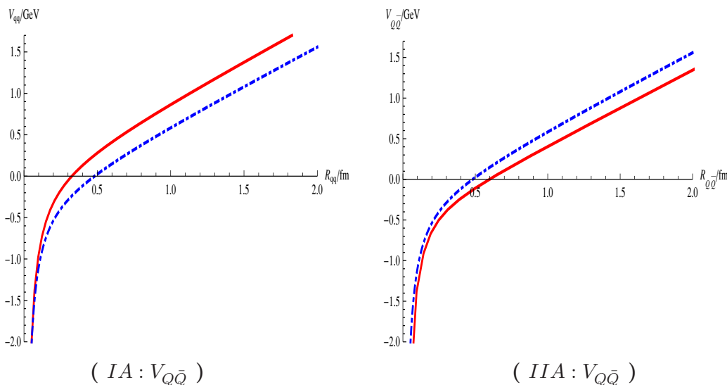
Figure 13. Heavy quark potential V_{Q\bar{Q}} as a function of R_{Q\bar{Q}} for Mod IA (with g_p = 2.2 ) and Mod IIA (with g_p = 2.8 ) are shown in solid lines compared with the Cornell potential shown in dot-dashed lines.
