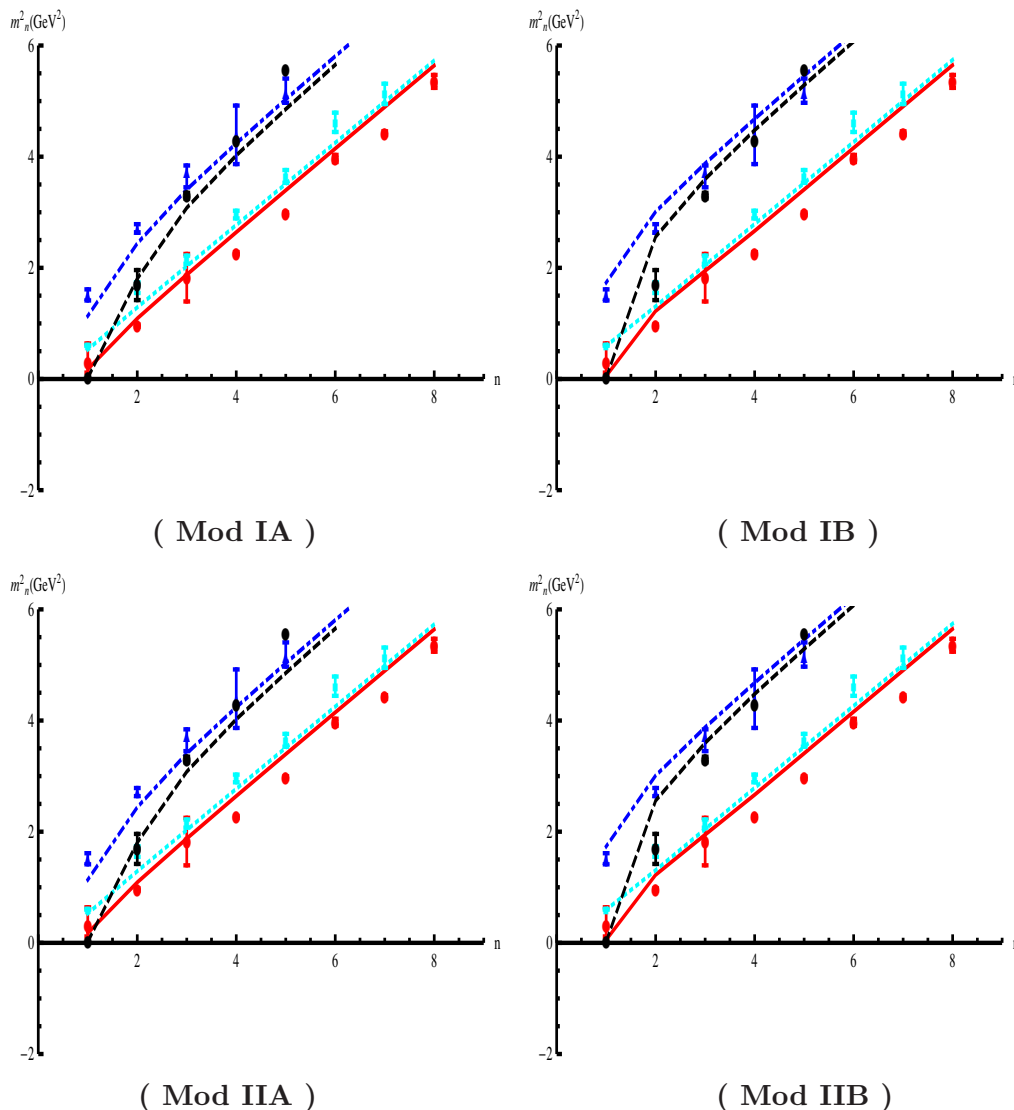
Figure 22. All meson spectra in Mod I and Mod II with two sets of parameters in table 7 comparing with experimental data.
