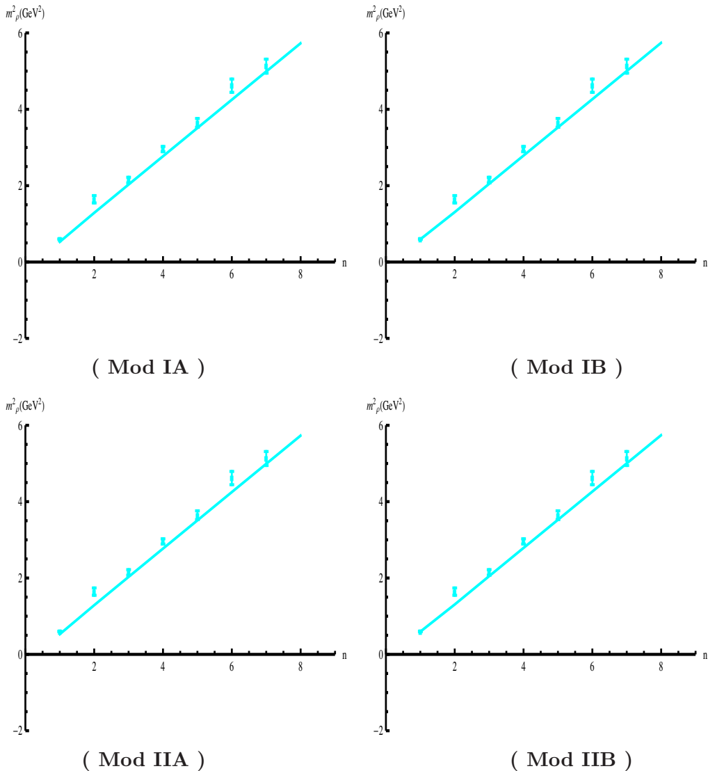
Figure 18. m_{\rho,n}^2 as functions of n for Mod I and II defined in table 7.
