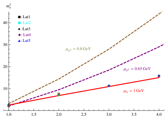
Figure 1. 0 ++ glueball in the dynamical soft-wall with quartic background \Phi = \mu_{G^2}^4 z^4 with \mu_{G^2} = 0.65, 0.8 GeV. The unit is in GeV, the dots are lattice data and the solid line is the result for quadratic background \Phi = \mu_G^2 z^2 with \mu_G = 1 GeV.
