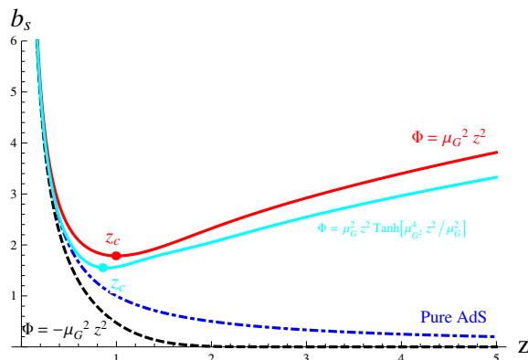
Figure 7. The metric structure b_s(z) = e^{A_s(z)} as functions of z corresponding to \Phi = \mu_G^2 z^2 (red solid line), \Phi = -\mu_G^2 z^2 (black dashed line), and \Phi = \mu_G^2 z^2 \tanh(\mu_G^4 z^2 / \mu_G^2) (cyan solid line), respectively. The blue dash-dotted line stands for the pure AdS 5 case. \mu_G = 1\text{GeV} has been taken for numerical calculation.
