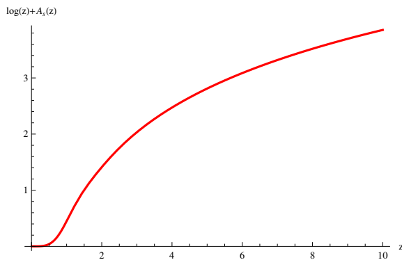
Figure 5. The deformed metric A_s as function of z for the dilaton field \Phi(z) = \mu_G^2 z^2 \tanh(\mu_{G^2}^4 z^2 / \mu_G^2) with \mu_G = \mu_{G^2} = 1\text{GeV} . Here we plot \log(z) + A_s(z) to avoid the \log(z) divergence at z = 0 of A_s which comes from the approximate AdS behavior of the solution.
