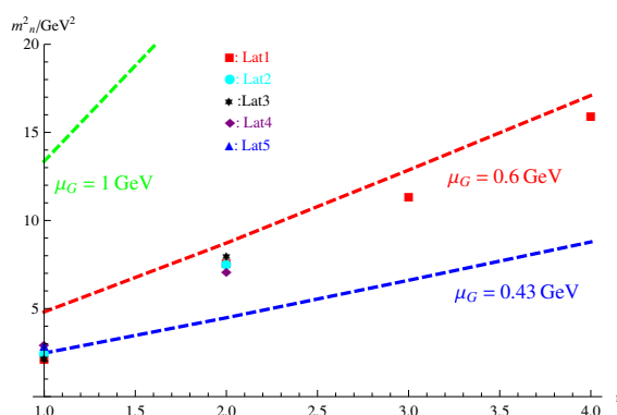
Figure 4. 0^{++} glueball in the dynamical soft-wall model with negative quadratic background \Phi = -\mu_G^2 z^2 with \mu_G = 0.43, 0.6, 1\text{ GeV} . The unit is in GeV and the dots are lattice data.
