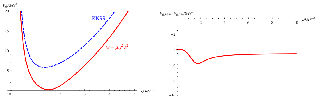
Figure 3. The potentials and their difference.
