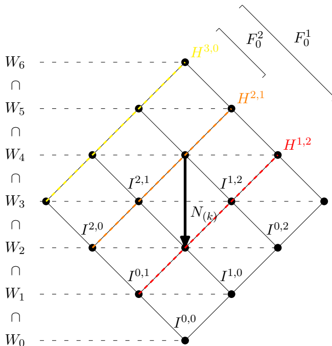
Figure 1. A Hodge-Deligne diamond illustrating how the spaces F_0^p , W_i , H^{p,q} and I^{p,q} are related. The arrow indicates a generic action of the log-monodromy matrix acting on these spaces.
