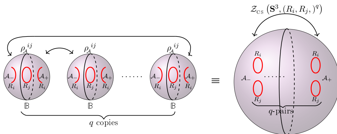
Figure 19. The replica computation for the density matrix \rho_{\mathcal{A}}^{ij} constructed in figure 18 glues q balls \mathbb{B} whose boundary is the union of \mathcal{A}_{\pm} for the chosen bipartition. As a result one ends up with a functional integral which computes \mathcal{Z}_{\text{CS}}(\mathbf{S}^3, (R_i, R_j)^q) \equiv \mathcal{Z}_{\text{CS}}(\mathbf{S}^3, R_i, R_j, \dots, R_i, R_j) , the \mathbf{S}^3 partition function with q -pairs of Wilson lines along unknots in representations R_i and R_j , respectively.
