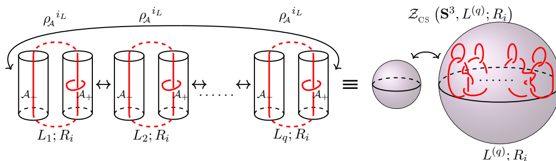
Figure 22. To compute the q^{\text{th}} -Rényi entropy for the reduced density matrix \rho_{\mathcal{A}}^{iL} we need to cyclically glue copies of the solid torii with a link L carrying representation R_i on each of its components. As indicated in figure 21 it is helpful to view this solid torus in terms of gluing together two solid cylinders with a link L contained within them. Gluing these together we see that we are required to compute the path integral over \mathbf{S}^3 with a Wilson line representation R_i placed along the direct sum of links L^{(q)} = L_1 + \dots + L_q . The q links get intertwined in the process of identifying the pieces of the density matrices across replica copies.
