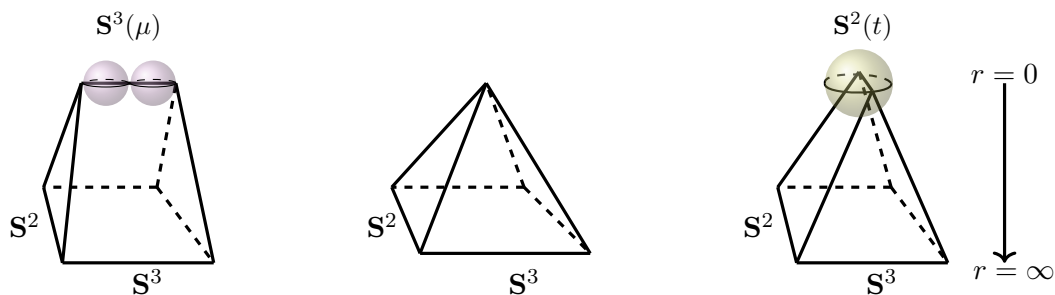
Figure 1. A illustration of the deformed, singular, and resolved conifold geometries viewed as a cone with a base that is topologically \mathbf{S}^2 \times \mathbf{S}^3 . We view the base as living far out along the cone r \rightarrow \infty , and the different topologies of the three geometries are captured by the behaviour near the tip. In the deformed conifold (left), \mathbf{S}^2 shrinks to a point and the \mathbf{S}^3 has radius \mu . The singular conifold (middle) instead has both the \mathbf{S}^3 and the \mathbf{S}^2 shrinking to a point at the tip. In the resolved conifold (right) on the other hand, the \mathbf{S}^3 shrinks to a point and the \mathbf{S}^2 has the Kähler parameter t . We have drawn the three-sphere as two 3-balls, which are to be identified along their boundaries. We will use this representation explicitly below, and also adhere to the color coding differentiating the three-ball \mathbb{B} from the two-sphere \mathbf{S}^2 (which will always be in yellowish hue).
