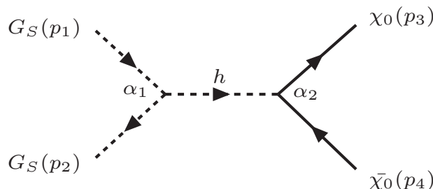
Figure 10. Feynman graph for pNGB ( G_s ) annihilation to neutralino ( \chi_0 ).
