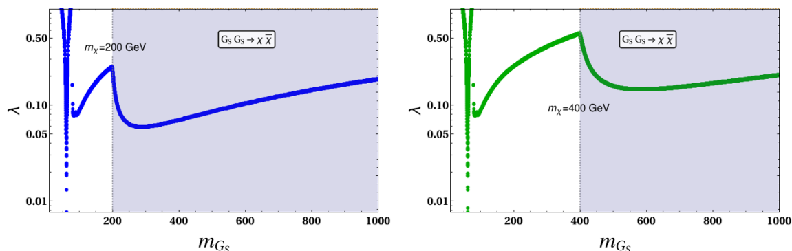
Figure 13. Region in the \lambda - m_{G_S} (in GeV) space allowed by the relic density constraint. We assumed all 15 pNBGs are degenerate and included the effects of the pNBG-LSP interaction with \tan\beta = 5 , C = 0.2 , and neutralino mass of m_{\chi_0} = 200 GeV (left) or m_{\chi_0} = 400 GeV (right).
