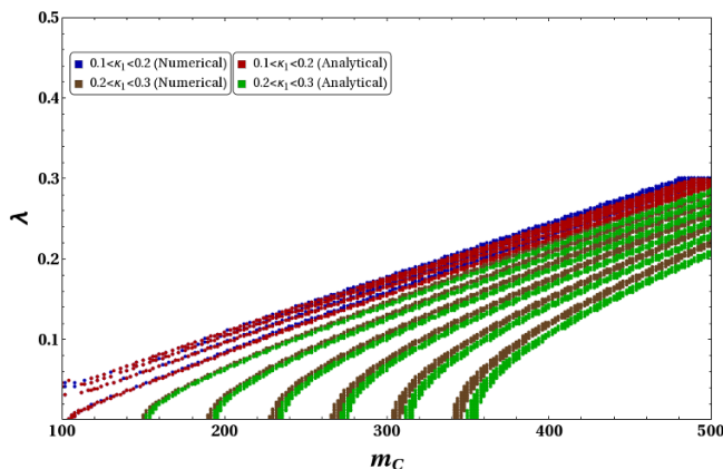
Figure 15. Comparison between relic density allowed points for C type pNGB ( \Omega_C h^2 < 1 ) found using numerical solution to coupled Boltzmann equation (eq. (C.3)) and approximate analytical solutions as in eq. (4.17) in m_C (GeV) - \lambda plane for \kappa : \{0.1 - 0.3\} .
