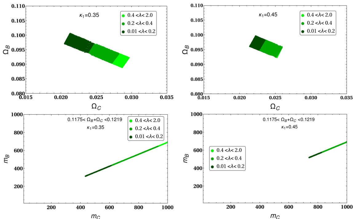
Figure 8. [Top panel:] Contribution to \Omega_T from \Omega_C and \Omega_B for different choices of \kappa_1 = 0.35 (left) and 0.45 (right). Different ranges of \lambda are indicated \lambda = \{0.01 - 0.2\} (dark green), \{0.2 - 0.4\} (green) and \{0.4 - 2.0\} (lighter green) respectively. [Bottom panel:] Mass correlation ( m_B - m_C ) in allowed relic density parameter space. Color codes remain the same as in top panel.
