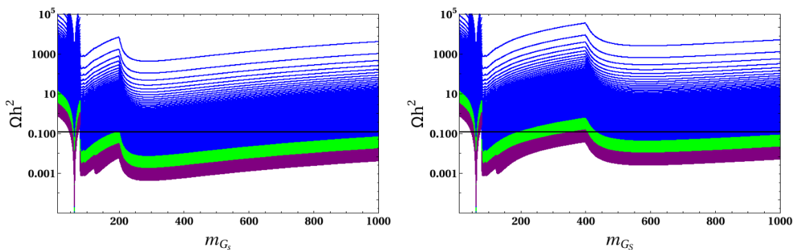
Figure 12. Relic density as a function of m_{G_S} (in GeV) for \lambda = 0.005 - 0.25 (blue), 0.25 - 0.5 (green) and 0.5 - 2 (purple). We assumed all 15 pNBGs are degenerate and included the effects of the pNBG-LSP interaction with \tan\beta = 5 , C = 0.2 , and a neutralino mass of m_{\chi_0} = 200 GeV (left) or m_{\chi_0} = 400 GeV (right).
