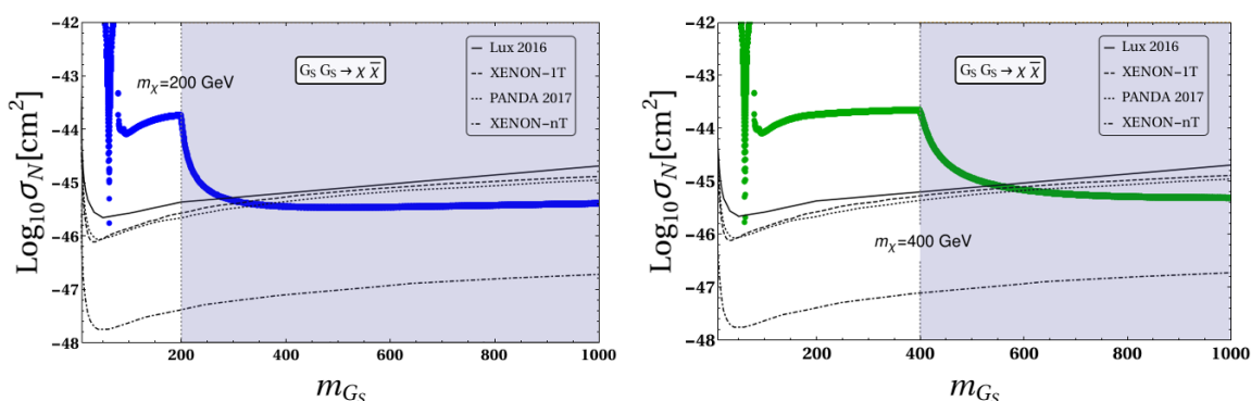
Figure 14. Direct search constraints for relic density allowed pNBG DM parameter space with non-negligible pNBG-neutralino interaction. LUX 2016 [54], XENON 1T [55], PANDA X [56] bounds and future prediction of XENONnT [57] are shown. MSSM parameters are chosen as \tan\beta = 5 , C = 0.2 and neutralino mass m_{\chi_0} = 200 GeV (left), m_{\chi_0} = 400 GeV (right).
