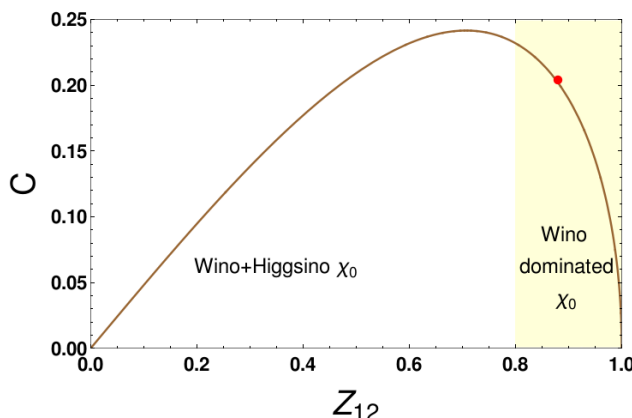
Figure 11. A plot between C and Z_{12} for \tan\beta = 5 assuming wino or wino-Higgsino dominated neutralino with Z_{11} = 0 and Z_{13} = Z_{14} . Our choice ( Z_{12} = 0.88 and C = 0.2 ) has been denoted by a red dot.
