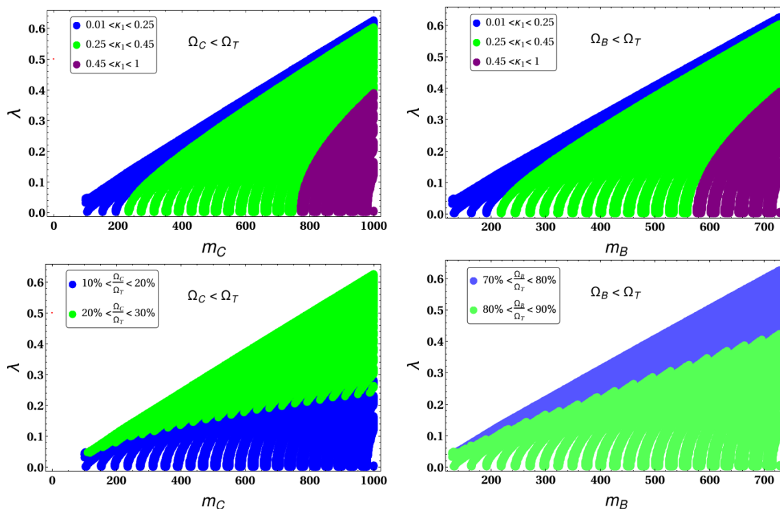
Figure 7. \lambda vs m_C (left) and \lambda vs m_B (right) for satisfying relic density 0.1175 < \Omega_T < 0.1219 . [Top panel:] Different choices of \kappa_1 are shown in different colours: 0.01 – 0.25 (blue), 0.25 – 0.45 (green), 0.45 – 1.0 (purple). [Bottom panel:] Relative contributions of individual DM candidates to total relic abundance have been shown in different colors.
