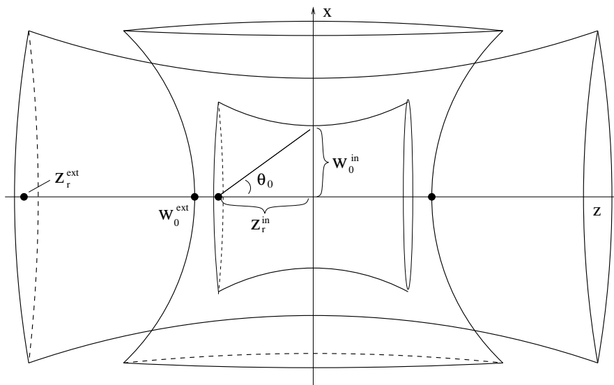
Figure 1. Spatial overlap of three focused laser beams at the coordinate center x = y = z = 0 . In this picture, the innermost beam gives the Gaussian probe beam embedded in two external beams which propagate orthogonally and transversally to it, respectively. The waist size w_0^{\text{ext}} as well as the Rayleigh lengths z_r^{\text{in}} and z_r^{\text{ext}} constitute scales for the extent of the beam foci along the propagation direction of the probe beam and thus parameterize the drop-off of the electric and magnetic field components of the lasers. The parameter \theta_0 = \frac{w_0}{z_r} is the aspect ratio for which typically \theta_0 \ll 1 .
