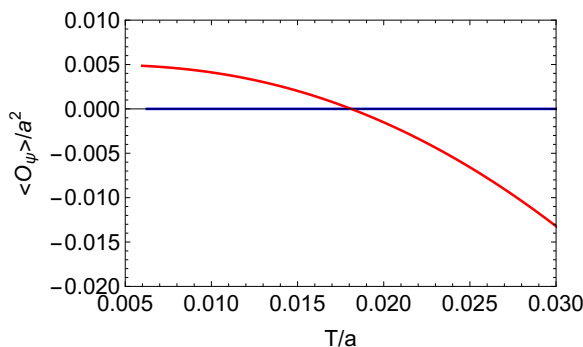
Figure 1: Plot showing the expectation value of the operator \mathcal{O}_\psi dual to the scalar field \psi (recall X = e^{-\psi/\sqrt{6}} ) for the black hole solutions. The blue line corresponds to the solution of [3], while the red lines indicate the two new branches of solution, one that exists for T \leq T_c and the other which appears to exist only for T \geq T_c .
