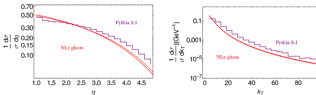
Figure 6. Collision energy \sqrt{s} = 13 TeV. Left: \eta -distribution after integrating over k_T in the range 4 \text{ GeV} < k_T < 100 \text{ GeV} . Right: k_T -distribution after integrating over \eta in the range 1 < \eta < 5 . Both distributions are normalized by the integrated cross-section over \eta and k_T in the ranges 4 \text{ GeV} < k_T < 100 \text{ GeV} and 1 < \eta < 5 .
