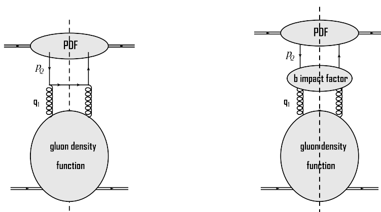
Figure 2. The same process as in figure 1 here presented as a convolution of the bottom quark impact factor and the gluon density.
