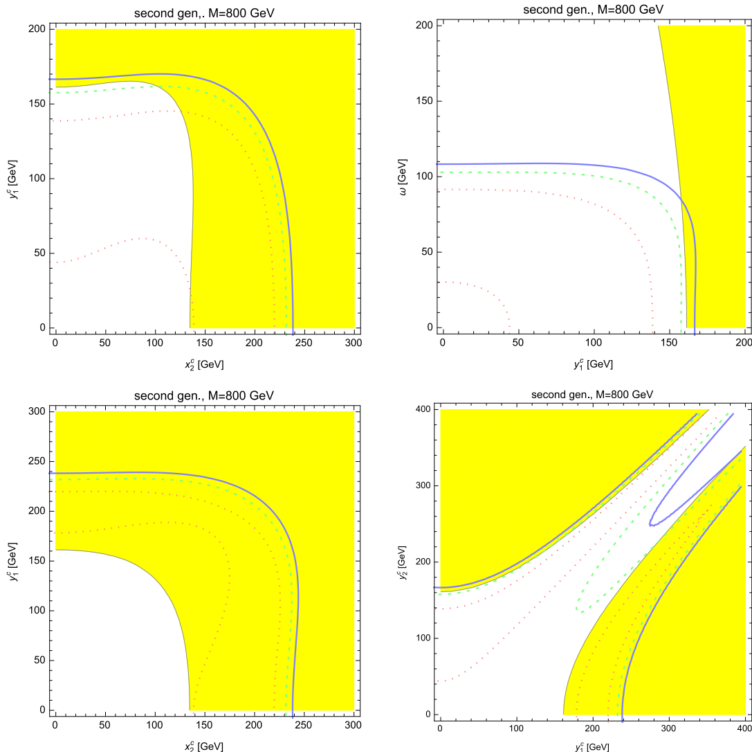
Figure 12. EWP bounds at 1\sigma (red-dashed), 2\sigma (green-dashed) and 3\sigma (blue) for VL quarks coupling with the second SM generations, compared with the region excluded at 3\sigma by tree-level bounds (yellow region in the left panel). We always chose M_1 = M_2 = M = 800 GeV and \omega = \omega' = 0 (except for the upper-right plot where \omega = \omega' \neq 0 ). Upper left panel: singlet Y = 2/3 and Doublet Y = 7/6 . Upper right panel: Doublet Y = 7/6 and Triplet Y = 5/3 . Lower left panel: singlet Y = 2/3 and Doublet Y = 1/6 . Lower right panel: Doublet Y = 1/6 and Doublet Y = 7/6 . Only the first quadrant is shown as the figures are symmetric with respect to a sign change in the coordinates in the other three quadrants. Note that in the four plots the variables and the units on the axis are not the same, so that they should not be compared directly as they refer to different multiplets.
