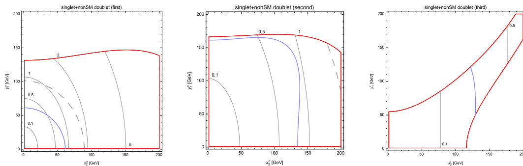
Figure 8. Singlet Y = 2/3 and Doublet Y = 7/6 for mixing with first generation only (left), second generation only (middle), third generation (right), and for a mass of the VL quarks of 800 GeV. The channel is T+jet . The grey contour lines correspond to cross-section values in picobarns at 14 TeV. The region inside the red line is allowed by the S and T parameters. The region inside the blue line is allowed by the tree-level bounds. The dashed black lines are the bounds from the ATLAS search [67].
