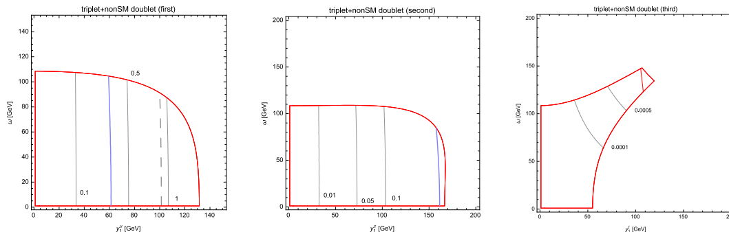
Figure 9. Doublet Y = 7/6 and Triplet Y = 5/3 for mixing with first generation only (left), second generation only (middle), third generation (right), and for a mass of the VL quarks of 800 GeV. The channel is T+jet. The grey contour lines correspond to cross-section values in picobarns at 14 TeV. The region inside the red line is allowed by the S and T parameters. The region inside the blue line is allowed by the tree-level bounds. The dashed black lines are the bounds from the ATLAS search [67].
