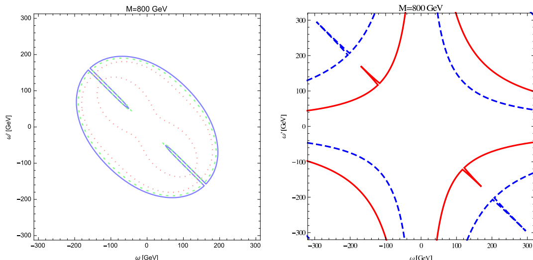
Figure 4. Doublet Y = 7/6 and Triplet Y = 5/3 (section 3.2). Left panel: EWP bounds at 1\sigma (red-dashed), 2\sigma (green-dashed) and 3\sigma (blue) as a function of the new Yukawa couplings \omega and \omega' with M = 800 GeV. In addition the mixing of VL quarks with SM quarks is taken to be zero i.e. y_1^k = 0 . Right panel: bound from ATLAS (blue) and CMS (red) data on Higgs couplings to photons and gluons.
