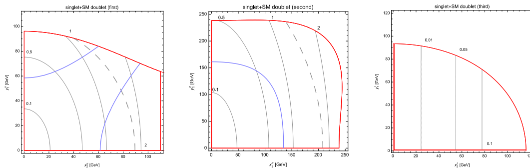
Figure 10. Singlet Y = 2/3 and Doublet Y = 1/6 for mixing with first generation only (left), second generation only (middle), third generation (right), and for a mass of the VL quarks of 800 GeV. The channel is T+jet. The grey contour lines correspond to cross-section values in picobarns at 14 TeV. The region inside the red line is allowed by the S and T parameters. The region inside the blue line is allowed by the tree-level bounds. The dashed black lines are the bounds from the ATLAS search [67].
