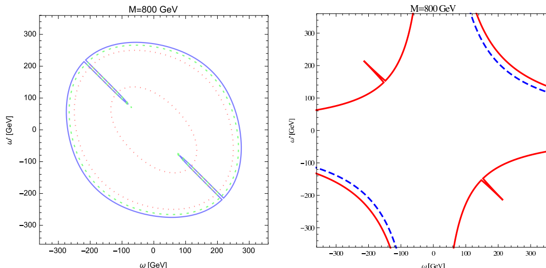
Figure 2. Singlet Y = 2/3 and Doublet Y = 7/6 (section 3.1). Left panel: EWP bounds at 1\sigma (red-dashed), 2\sigma (green-dashed) and 3\sigma (blue) as a function of the new Yukawa couplings \omega and \omega' with M = 800 GeV. We have assumed that there is no mixing of VL quarks with the SM quark generations i.e. x_2^k = y_1^k = 0 . Right panel: bound from ATLAS (dashed blue) and CMS (solid red) data on Higgs couplings to photons and gluons.
