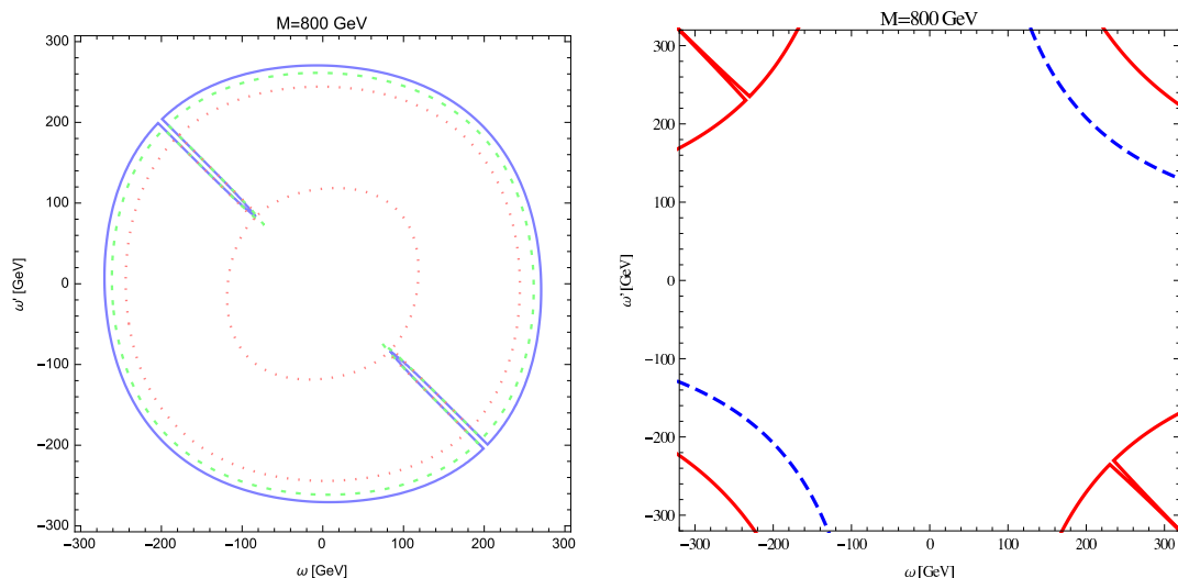
Figure 6. Singlet Y = 2/3 and Doublet Y = 1/6 (section 3.3). Left panel: EWP bounds at 1\sigma (red-dashed), 2\sigma (green-dashed) and 3\sigma (blue) as a function of the new Yukawa couplings \omega and \omega' with M = 800 GeV. In addition the mixing of VL quarks with SM quarks is taken to be zero i.e. y_1^k = 0 . Right panel: bound from ATLAS (blue) and CMS (red) data on Higgs couplings to photons and gluons.
