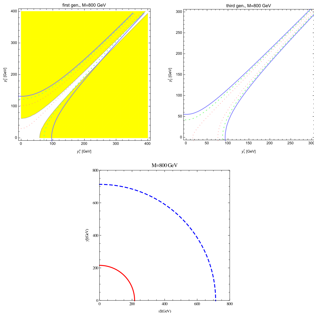
Figure 7. Doublet Y = 1/6 and Doublet Y = 7/6 (section 3.4). EWP bounds at 1\sigma (red-dashed), 2\sigma (green-dashed) and 3\sigma (blue) for VL quarks coupling with the first (top left panel) and third (to right panel) SM generations, compared with the region excluded at 3\sigma by tree-level bounds (yellow region in the left panel). Bottom panel: bounds from ATLAS (dashed blue) and CMS (solid red) data on Higgs couplings to photons and gluons considering VL couplings with first SM generation. Plot for the coupling of VL quarks with second SM generation is similar.
