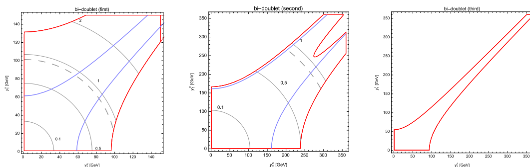
Figure 11. Doublet Y = 1/6 and Doublet Y = 7/6 for mixing with first generation only (left), second generation only (middle), third generation (right), and for a mass of the VL quarks of 800 GeV. The channel is T+jet. The grey contour lines correspond to cross-section values in picobarns at 14 TeV (this channel is not allowed in the case of the plot on the right). The region inside the red line is allowed by the S and T parameters. The region inside the blue line is allowed by the tree-level bounds. The dashed black lines are the bounds from the ATLAS search [67].
