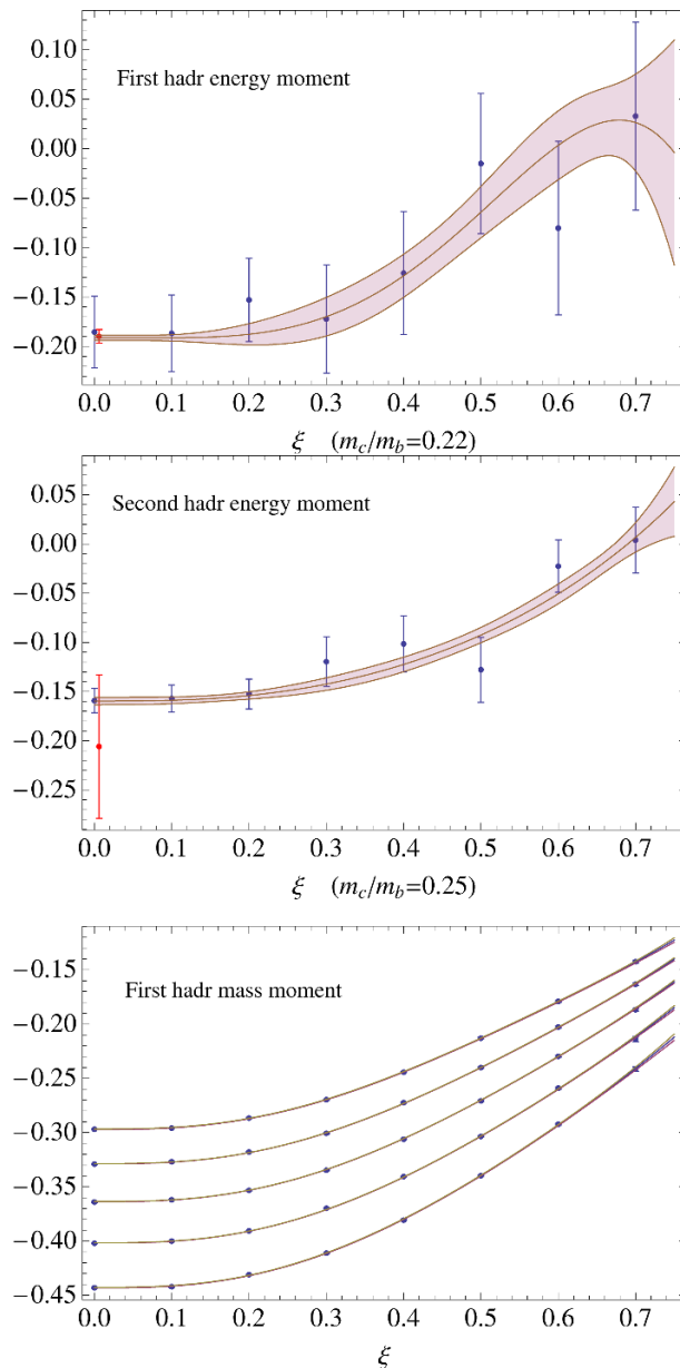
Figure 5. Combinations of two-loop non-BLM contributions \chi_{01}^{(2)} , \chi_{02}^{(2)} , and \chi_{10}^{(2)} entering the hadronic moments: numerical evaluation [21] with blue errors and analytic one [19, 20] at \xi = 0 with red errors vs. fits (shaded bands). \chi_{10}^{(2)} (lower panel) is shown for r = 0.2, 0.22, 0.24, 0.26, 0.28 .
