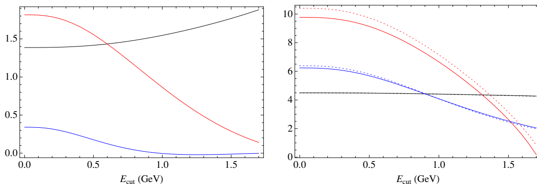
Figure 6. E_{cut} dependence of leptonic (left) and hadronic (right) at NNLO in the kinetic scheme with \mu = \mu_c = 1\text{GeV} . The black, red, blue lines refer to \ell_1, 10 \times \ell_2, -10 \times \ell_3 and to h_1, 8 \times h_2, h_3 , respectively, each expressed in \text{GeV} to the appropriate power. The dotted lines (indistinguishable for the leptonic moments) represent the predictions at O(\alpha_s^2\beta_0) .
