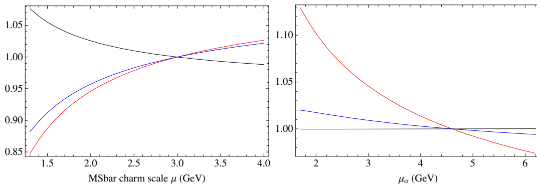
Figure 8. Dependence of h_{1,2,3} at E_{cut} = 0 on a ) the charm \overline{\text{MS}} scale \bar{\mu} (left panel) and b ) the scale of \alpha_s when the kinetic scheme is applied to m_c as well (right panel). The moments are normalized to their values at \bar{\mu} = 3 \text{ GeV} and \mu_\alpha = m_b , respectively. The kinetic cutoff is fixed at 1 GeV. The black, red, blue lines refer to h_{1,2,3} .
