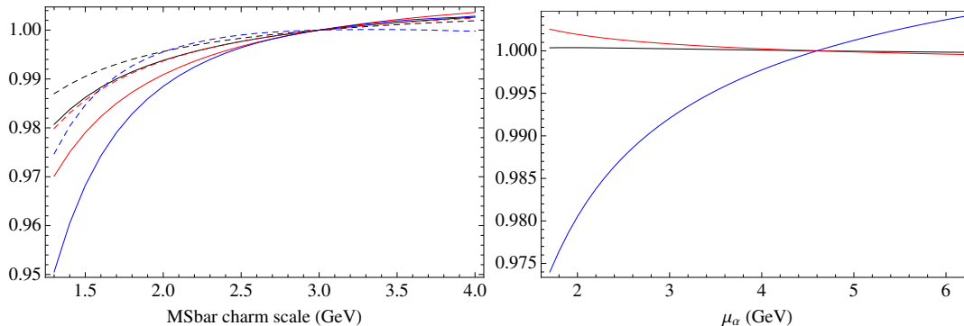
Figure 4. Dependence of the first three leptonic central moments at E_{cut} = 0 on a ) the charm \overline{\text{MS}} scale \bar{\mu} (left panel) and b ) the scale of \alpha_s when the kinetic scheme is applied to m_c as well (right panel). The moments are normalized to their values at \bar{\mu} = 3 \text{ GeV} and \mu_\alpha = m_b , respectively. The kinetic cutoff is fixed at 1 GeV. The black, red, blue lines refer to \ell_{1,2,3} . The solid (dashed) lines refer to four (two) loop evolution.
