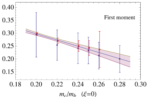
Figure 2. The non-BLM contribution \eta_1^{(2)}(\xi = 0) to the first leptonic moment as a function of r : numerical evaluation [21] with blue errors and analytic one [19, 20] at \xi = 0 with red errors vs. fits (shaded bands).
