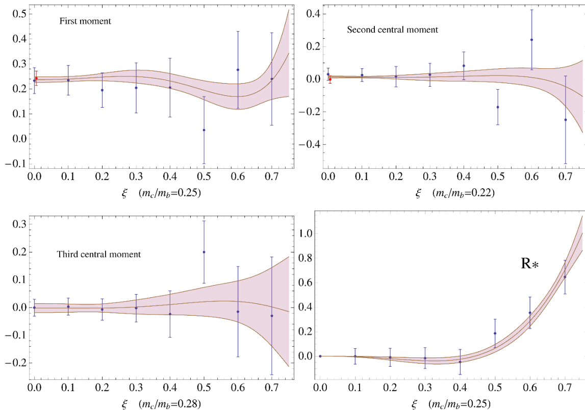
Figure 1. Combinations of two-loop non-BLM contributions entering the normalized central leptonic moments and R^* : numerical evaluation [21] with blue errors and analytic one [19, 20] at \xi = 0 with red errors vs. fits (shaded bands).
