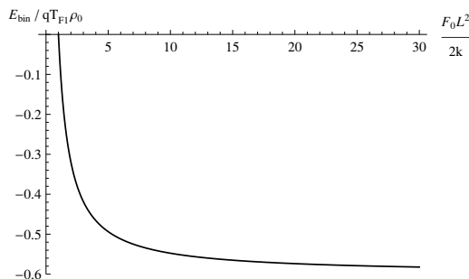
Figure 7. Binding energy per string of the di-monopole, in units of T_{F1} \rho_0 , as a function of \frac{F_0 L^2}{2k} .
