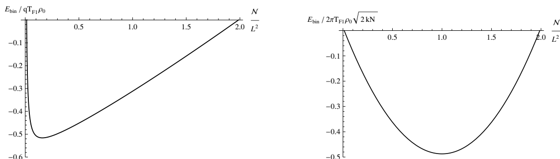
Figure 3. Binding energy per string (left) and total binding energy (right) of the di-baryon (in units of T_{F1} \rho_0 and 2\pi T_{F1} \rho_0 \sqrt{2k\mathcal{N}} respectively) as a function of \mathcal{N}/L^2 .
