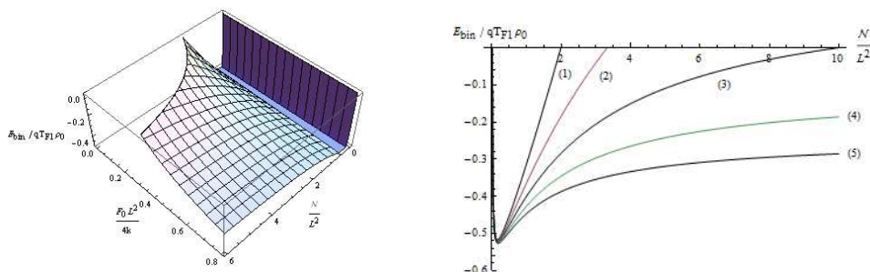
Figure 9. Binding energy per string for the di-baryon, in units of T_{F1} \rho_0 , as a function of the magnetic flux and the mass (right: \frac{F_0 L^2}{4k} = \{0, 0.2, 0.4, 0.6, 0.8\} for (1)-(5) respectively).
