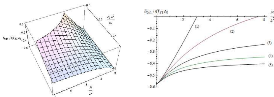
Figure 10. Binding energy per string for the baryon vertex, in units of T_{F1} \rho_0 , as a function of the magnetic flux and the mass (right: \frac{F_0 L^2}{6k} = \{0, 0.2, 0.4, 0.6, 0.8\} for (1)-(5) respectively).
