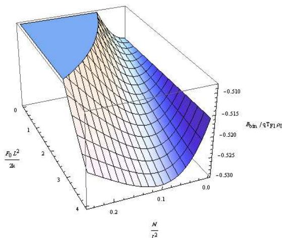
Figure 8. Binding energy per string of the 't Hooft monopole, in units of T_{F1} \rho_0 , as a function of the magnetic flux and the mass.
