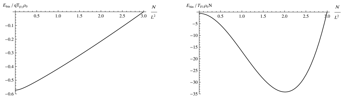
Figure 5. Binding energy per string (left) and total binding energy (right) of the baryon vertex (in units of T_{F1} \rho_0 and T_{F1} \rho_0 N respectively) as a function of \mathcal{N}/L^2 .
