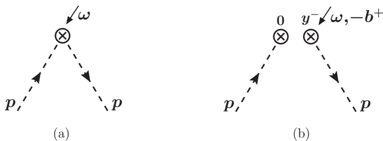
Figure 3. Tree-level diagram for the quark PDF (a) and the quark beam function (b). For the latter, the y^- coordinate separation in the operator is indicated by drawing separated vertices for each field.
