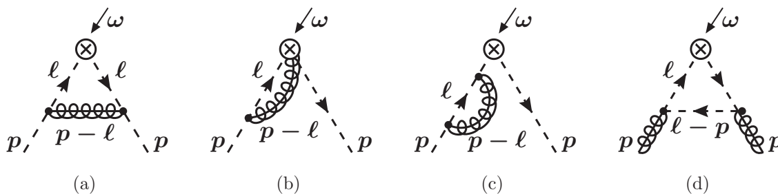
Figure 5. Nonzero one-loop diagrams for the quark PDF. The minus momentum \omega enters the vertex through its outgoing fermion line and leaves through its incoming fermion line. Diagram (c) represents the inclusion of the wave-function renormalization constant for the renormalized fields together with the corresponding residue factor in the LSZ formula for the S -matrix. Diagrams (b) and (c) have symmetric counterparts which are included in their computation.
