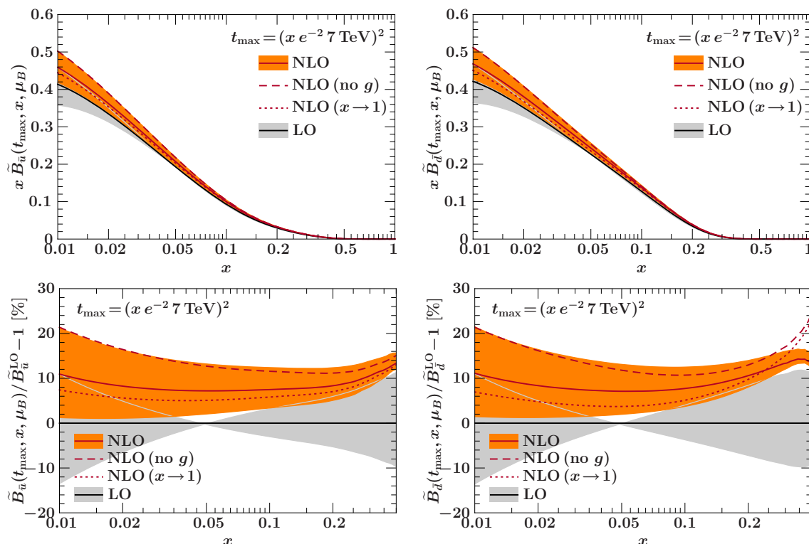
Figure 9. The \bar{u} (left column) and \bar{d} (right column) beam functions at the beam scale. The meaning of the curves is analogous to figure 8.
