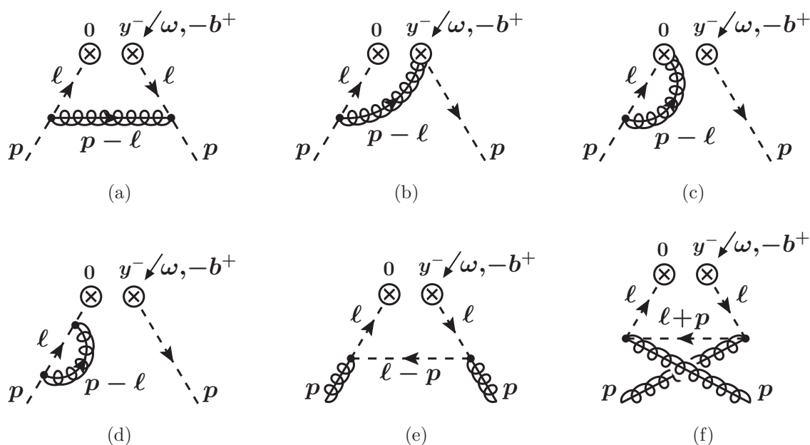
Figure 6. One-loop diagrams for the quark beam function. The minus momentum \omega is incoming at the vertex and the b^+ momentum is outgoing. Diagram (d) denotes the wave-function contribution. Diagrams (b), (c), and (d) have symmetric counterparts which are equal to the ones shown and included in the computation. Diagram (f) and the diagram with the gluon connecting both vertices vanish.
