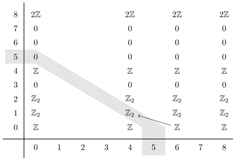
Figure 10. E_2 page of the AHSS for \Omega_*^{\text{Spin}}(BSU(n)) . We have shaded the entries contributing to the computation of \Omega_5^{\text{Spin}}(BSU(n)) , and indicated the only relevant differential.
