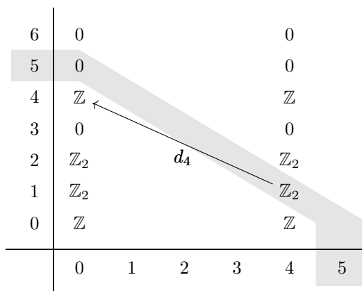
Figure 7. E_4 page of the AHSS for \Omega_*^{\text{Spin}}(BSU(2)) . We have shaded the entries of total degree 5, and indicated explicitly the only potentially non-vanishing differential acting on the shaded region.
