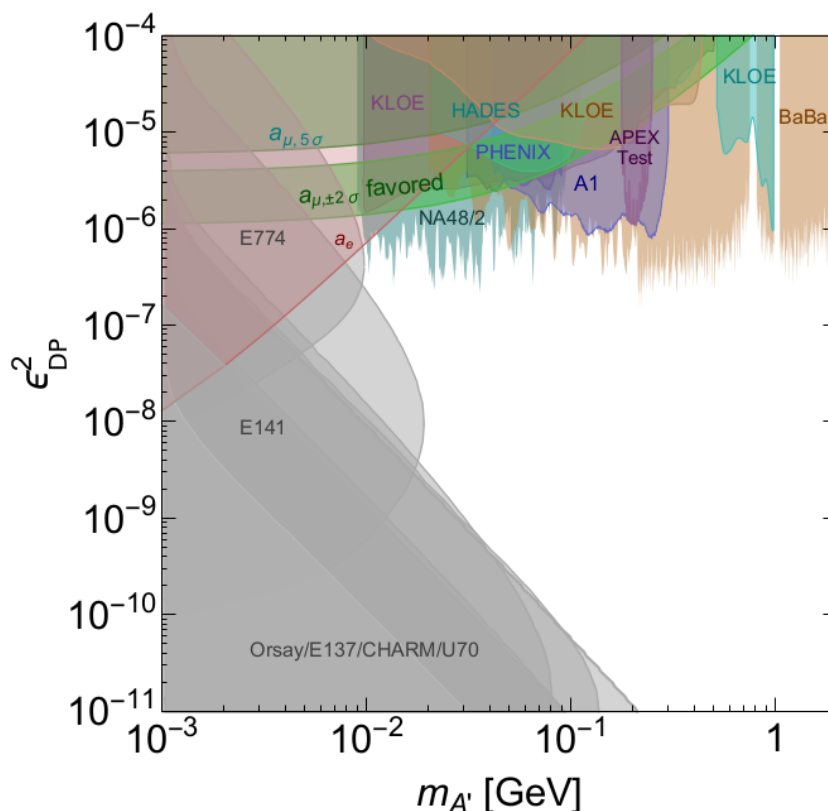
Figure 10. Summary of bounds from low energy accelerators constraints on the dark photon model [110]. After proper rescaling these constraints are also applicable to the U(1)_X models in this work. In particular, the BaBar limits can be recast using the relation \epsilon_{\text{DP}}^2 \rightarrow (g_v^l)^2 BR(Z' \rightarrow l^+l^-) . See text for details.
