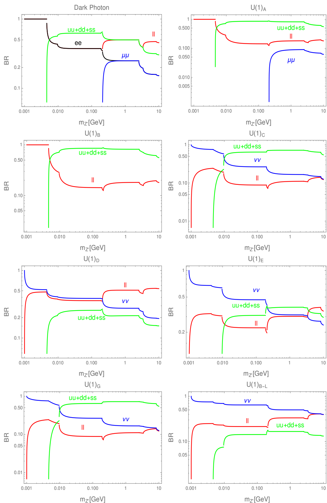
Figure 1. Branching ratios as a function of the Z' mass for several U(1)_X models under study.
