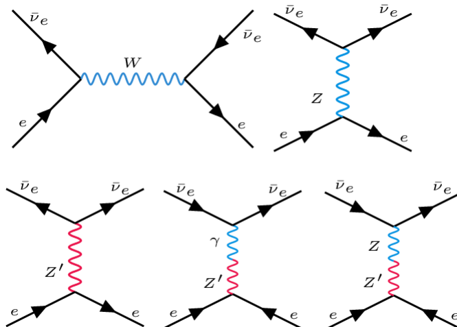
Figure 7. Feynmann diagrams relevant for neutrino-electron scattering.
