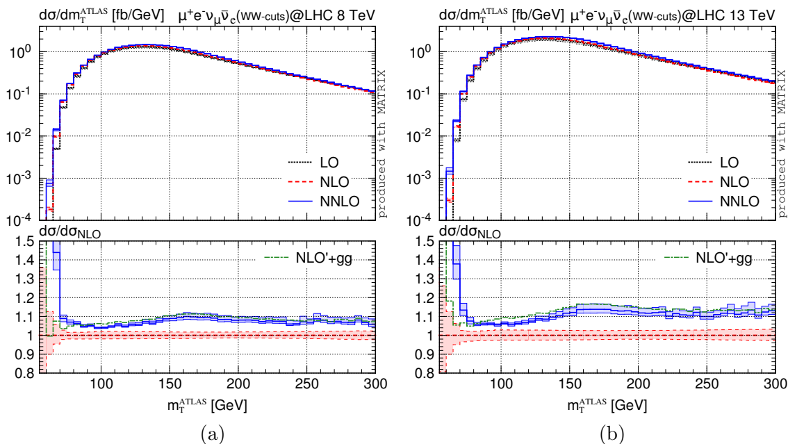
Figure 11. Distribution in the W^+W^- transverse mass. W^+W^- cuts are applied. Absolute predictions and relative corrections as in figure 4.
