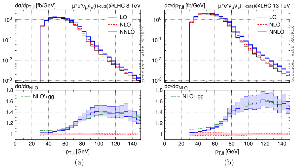
Figure 22. Distribution in the p_T of the dilepton system. Higgs cuts are applied. Absolute predictions and relative corrections as in figure 4.
