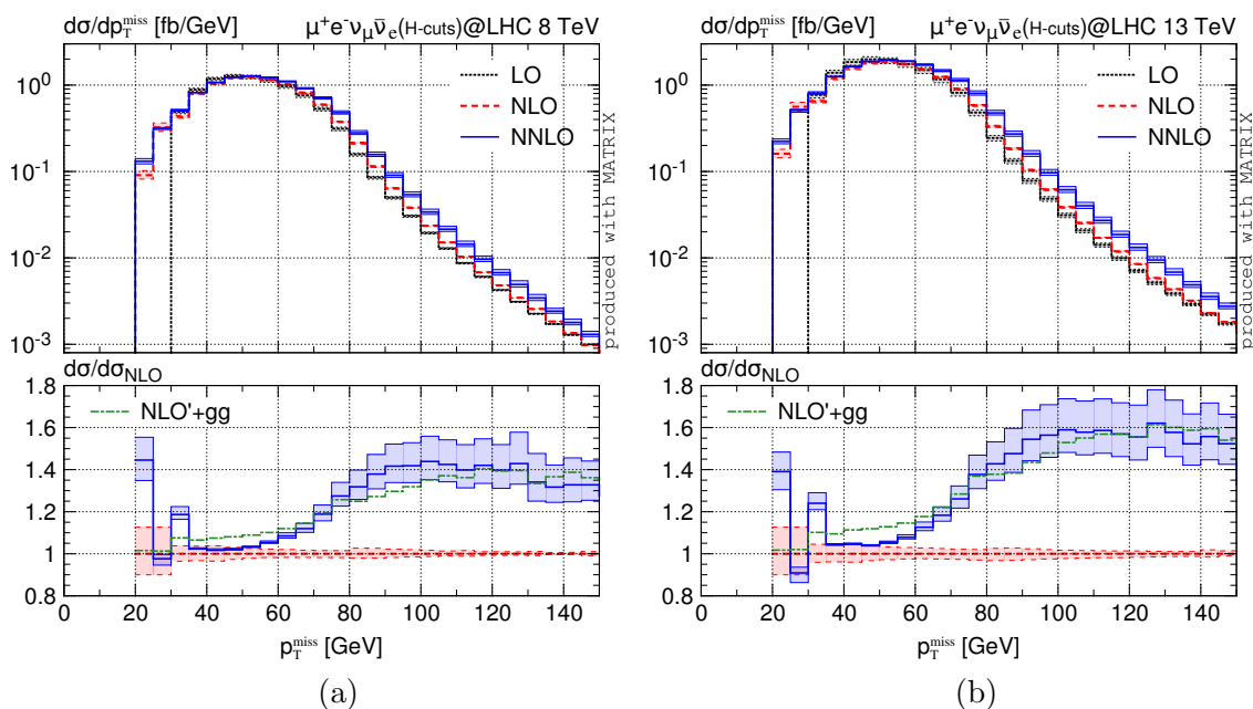
Figure 23. Distribution in the missing transverse momentum. Higgs cuts are applied. Absolute predictions and relative corrections as in figure 4.
