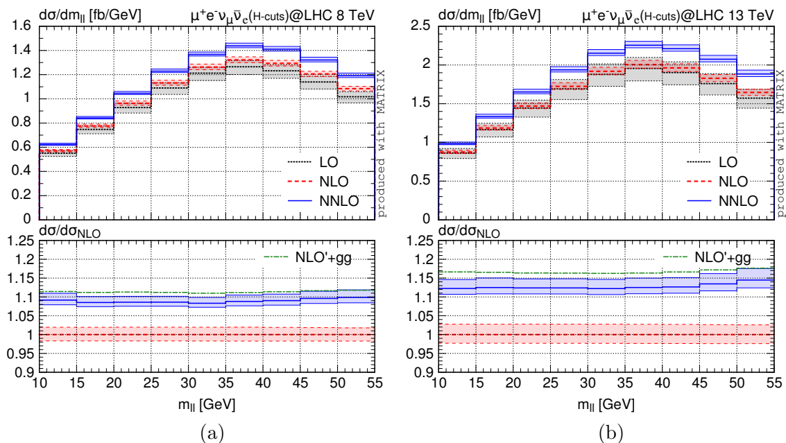
Figure 18. Distribution in the dilepton invariant mass. Higgs cuts are applied. Absolute predictions and relative corrections as in figure 4.
