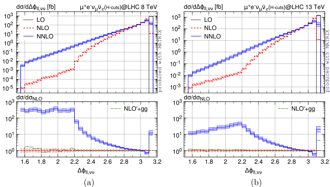
Figure 17. Distribution in the azimuthal separation between the transverse momentum of the dilepton system and the missing transverse momentum. Higgs cuts are applied. Absolute predictions and relative corrections as in figure 4.
