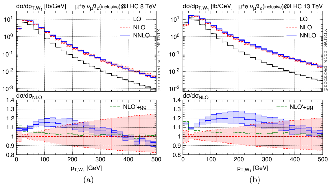
Figure 6. Distribution in the transverse momentum of the harder reconstructed W boson. No acceptance cuts are applied. Absolute predictions and relative corrections as in figure 4.
