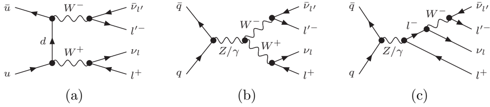
Figure 1. Sample of Born diagrams contributing to W^+W^- production both in the different-flavour case ( l \neq l' ) and in the same-flavour case ( l = l' ).
