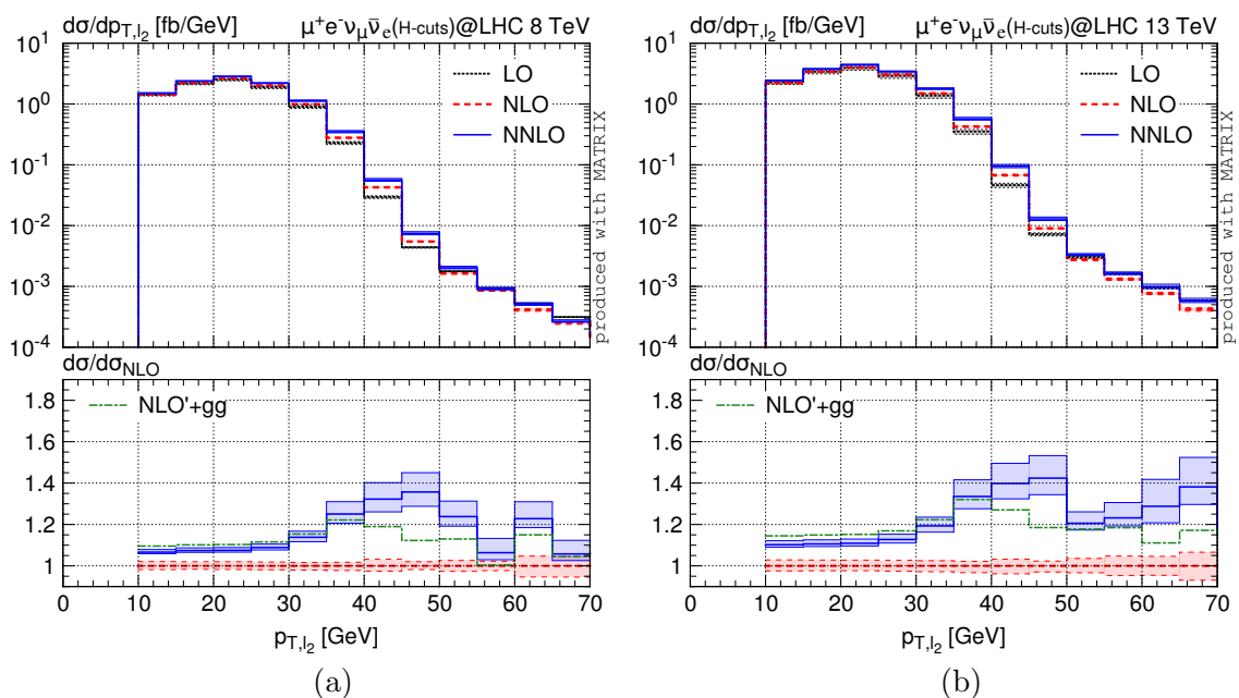
Figure 21. Distribution in the p_T of the subleading lepton. Higgs cuts are applied. Absolute predictions and relative corrections as in figure 4.
