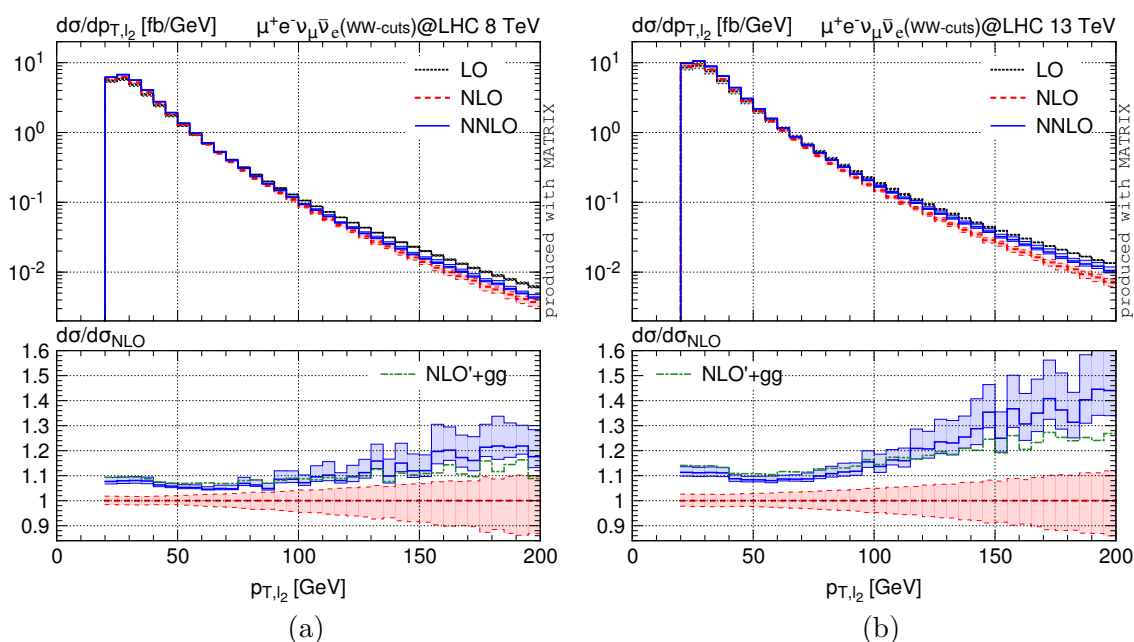
Figure 13. Distribution in the p_T of the subleading lepton. W^+W^- cuts are applied. Absolute predictions and relative corrections as in figure 4.
