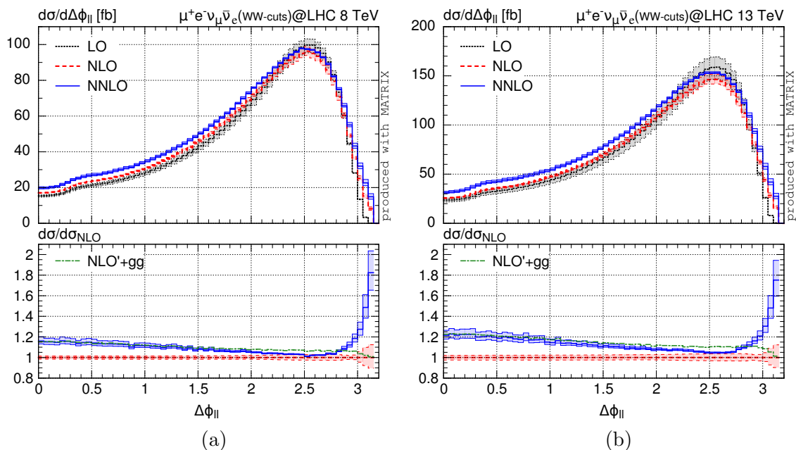
Figure 8. Distribution in the azimuthal separation of the charged leptons. W^+W^- cuts are applied. Absolute predictions and relative corrections as in figure 4.
