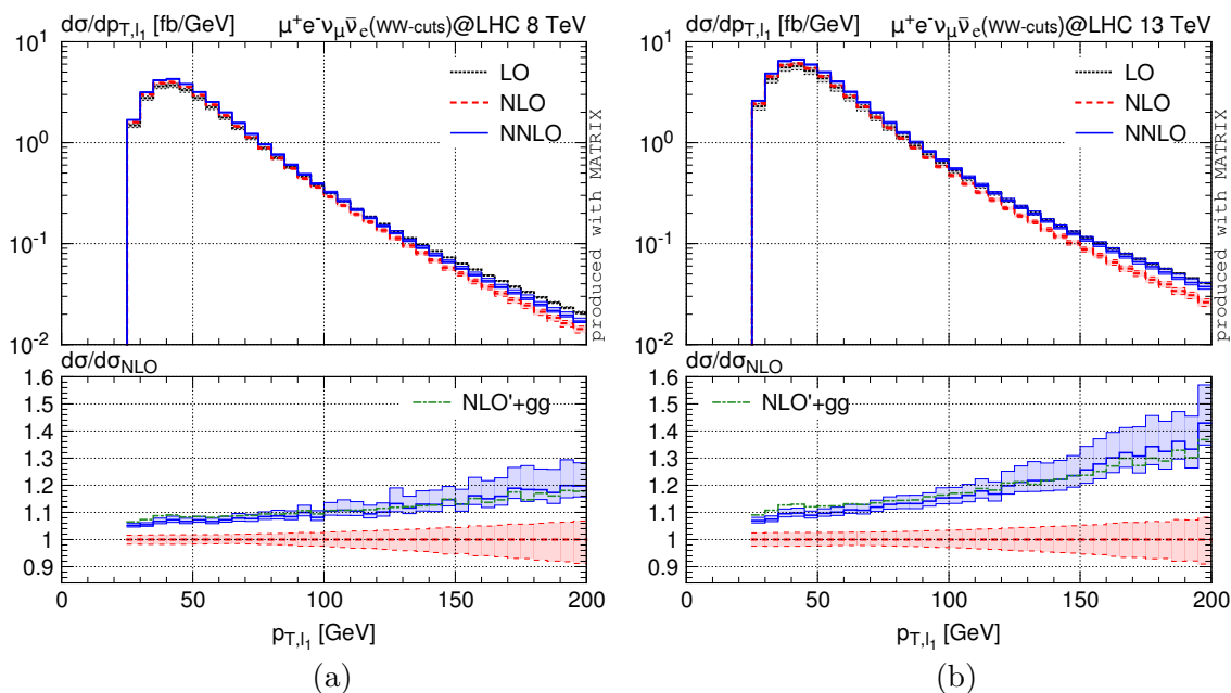
Figure 12. Distribution in the p_T of the leading lepton. W^+W^- cuts are applied. Absolute predictions and relative corrections as in figure 4.
