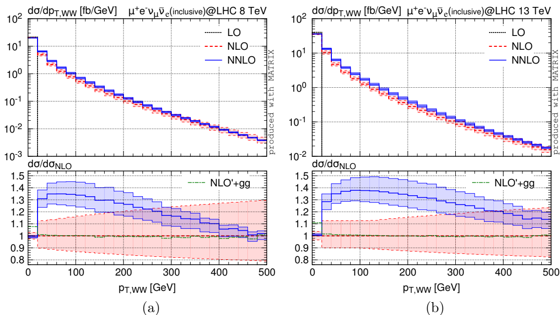
Figure 5. Distribution in the transverse momentum of the W^+W^- pair. No acceptance cuts are applied. Absolute predictions and relative corrections as in figure 4.
