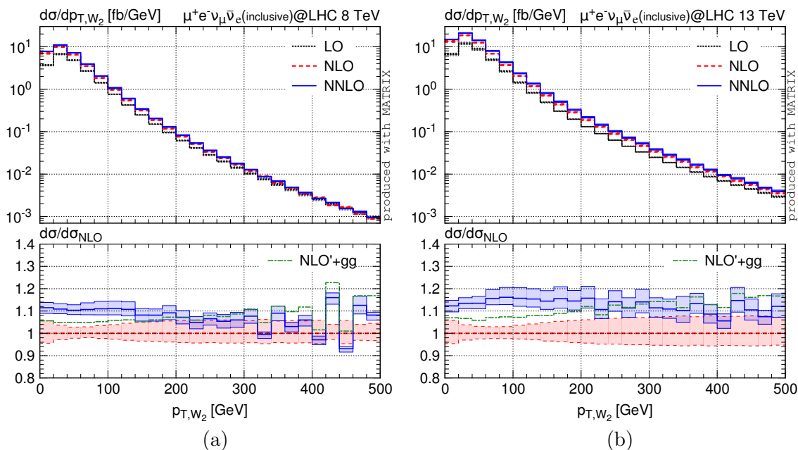
Figure 7. Distribution in the transverse momentum of the softer reconstructed W boson. No acceptance cuts are applied. Absolute predictions and relative corrections as in figure 4.
