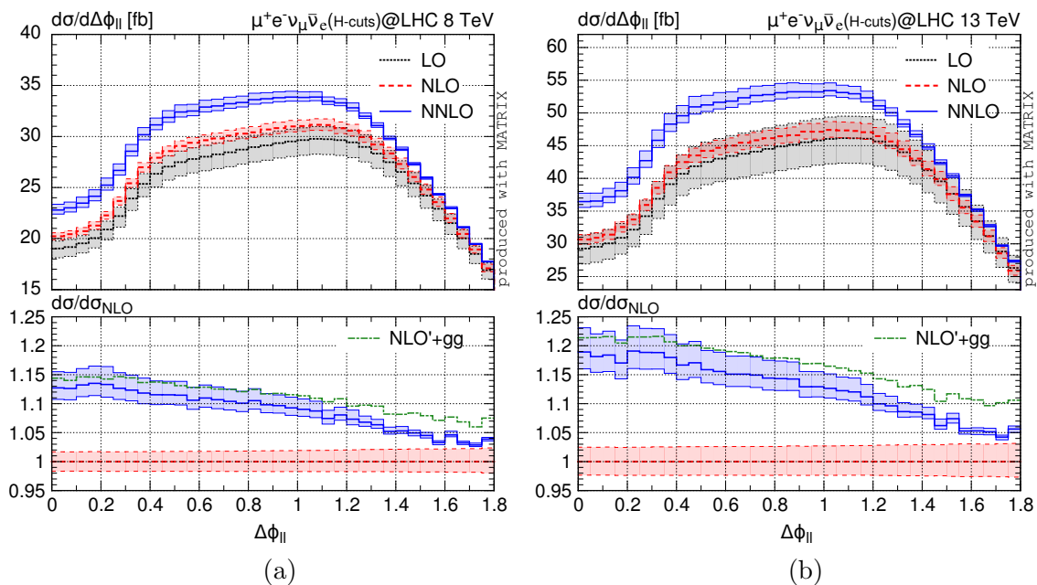
Figure 16. Distribution in the azimuthal separation of the charged leptons. Higgs cuts are applied. Absolute predictions and relative corrections as in figure 4.
