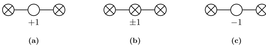
Figure 1. Three Dynkin diagrams for \mathfrak{psu}(1,1|2) .
