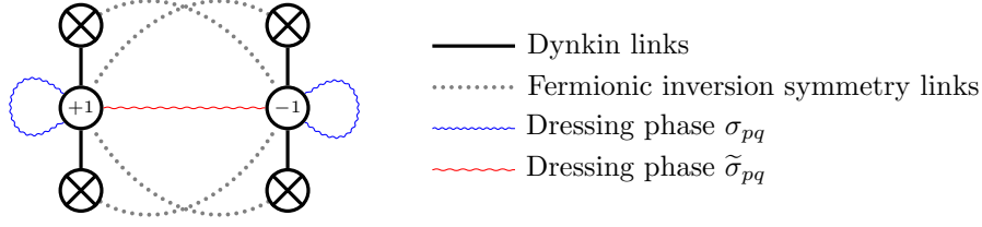
Figure 3. The Dynkin diagram for \mathfrak{psu}(1,1|2)^2 with the various interaction terms appearing in the Bethe ansatz indicated. The label \pm 1 inside the middle Dynkin nodes indicate the \mathfrak{su}(2) and \mathfrak{sl}(2) gradings of the left- and right-moving sectors.
