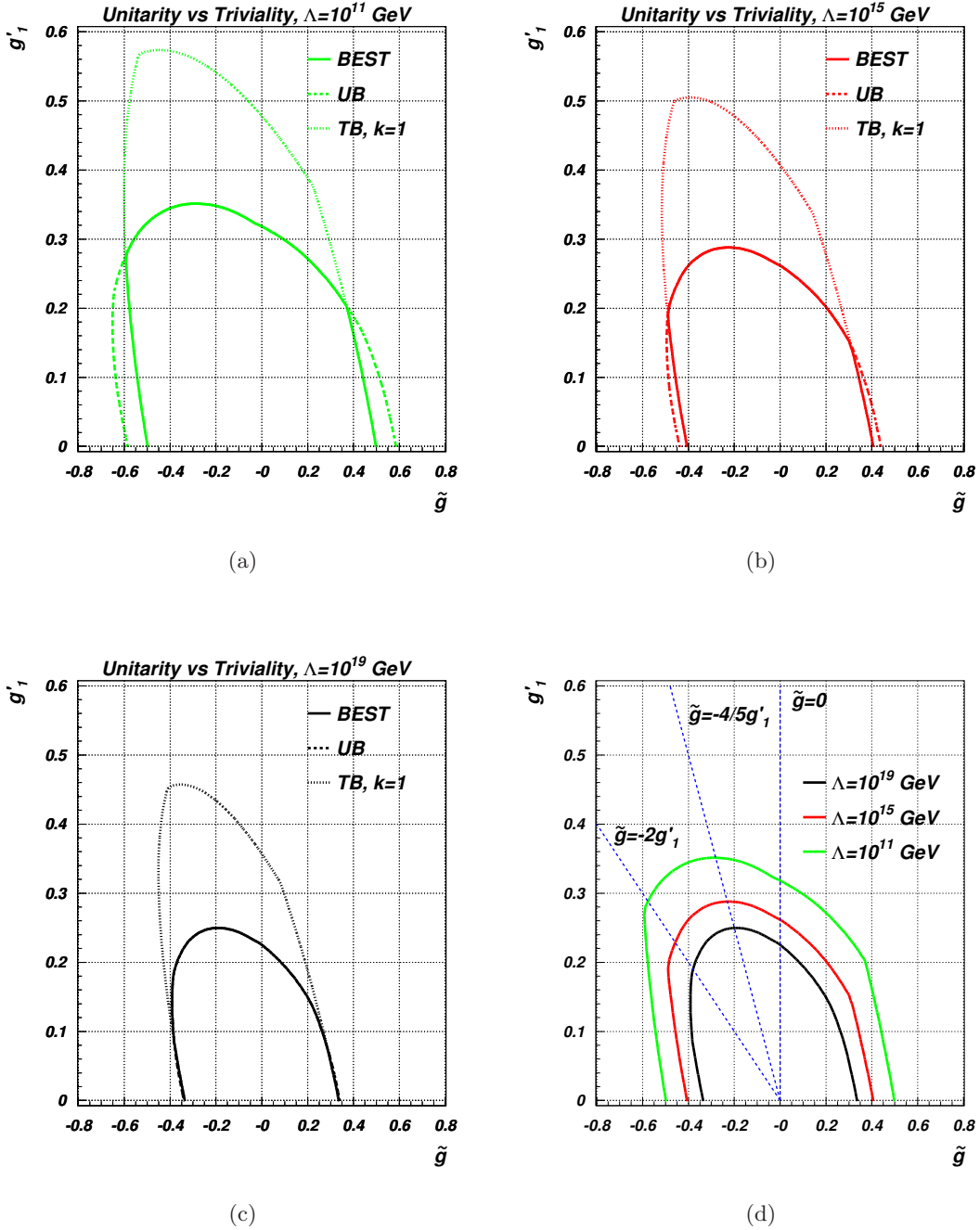
Figure 1: Contour plot of both the greater eigenvalue of the spherical wave scattering matrix (table 2) allowed by unitarity (dashed lines) and the gauge couplings allowed by triviality (dotted lines) for several values of the cut-off energy: \Lambda = 10^{11} GeV (light green/grey lines, figure 1a), \Lambda = 10^{15} GeV (dark red/grey lines, figure 1b), \Lambda = 10^{19} GeV (black lines, figure 1c). Figure 1d shows a summary of the most stringent bounds at different values of the cut-off energy, with focus on some peculiar parametrisation of \tilde{g} (table 1).
