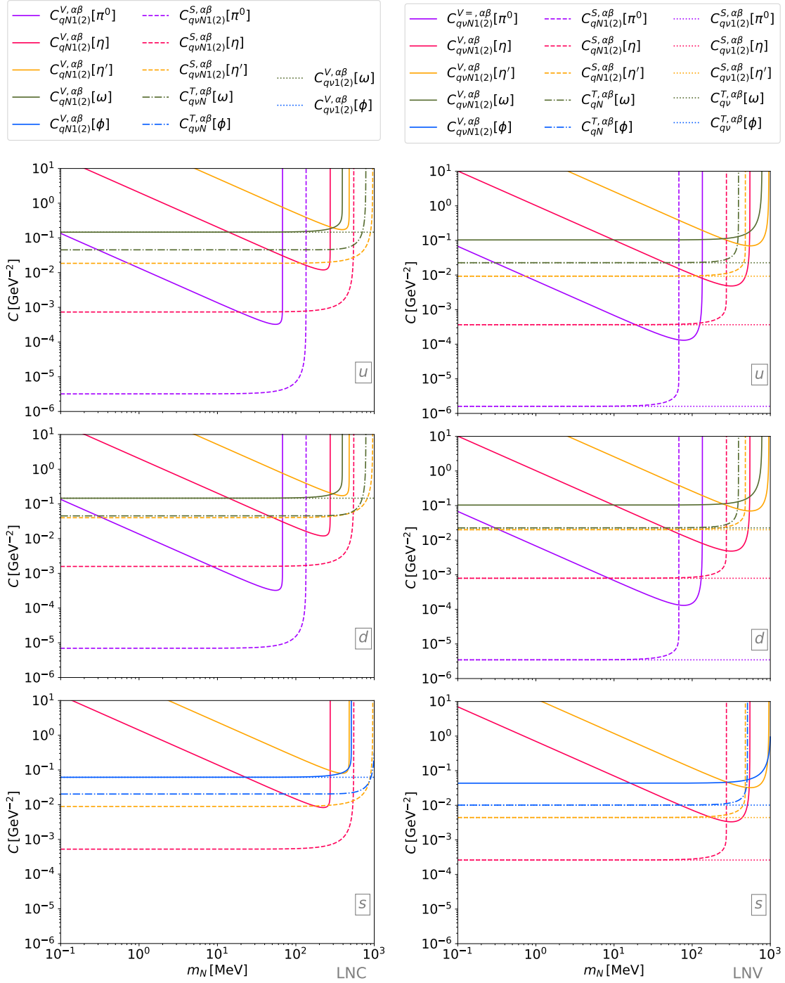
Figure 2. Upper bounds on the LNEFT Wilson coefficients of dim-6 neutrino-quark operators from meson invisible decays as a function of m_N for LNC (LNV) operators on the left (right). The top (middle) [bottom] row show WCs for up (down) [strange] quarks. For the LNV WCs C_{qv1(2)}^{S, \alpha\beta} , C_{qN1(2)}^{S, \alpha\beta} we display the components with \alpha \neq \beta . The bounds for the corresponding WCs with \alpha = \beta are stronger by a factor \sqrt{2} .
