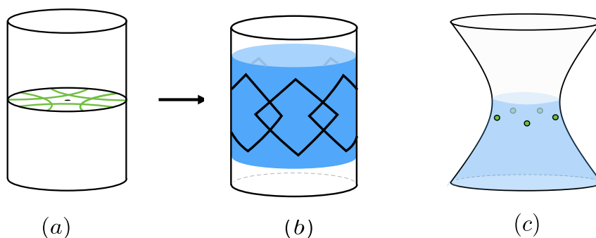
Figure 12. (a) A bulk local operator is recovered from an integral over bulk geodesic operators. (b) The boundary representation is a corresponding integral over diamond-smeared operators. The result is a smeared representation of the bulk local operator that is supported on a time-interval of the cylinder tiled by these diamonds. (c) For each geodesic, we chose the causal diamond that subtends less than half the circle. The domain of integration is the lower-half of the kinematic space for the hyperbolic plane. A few corresponding examples are shown in each panel.
