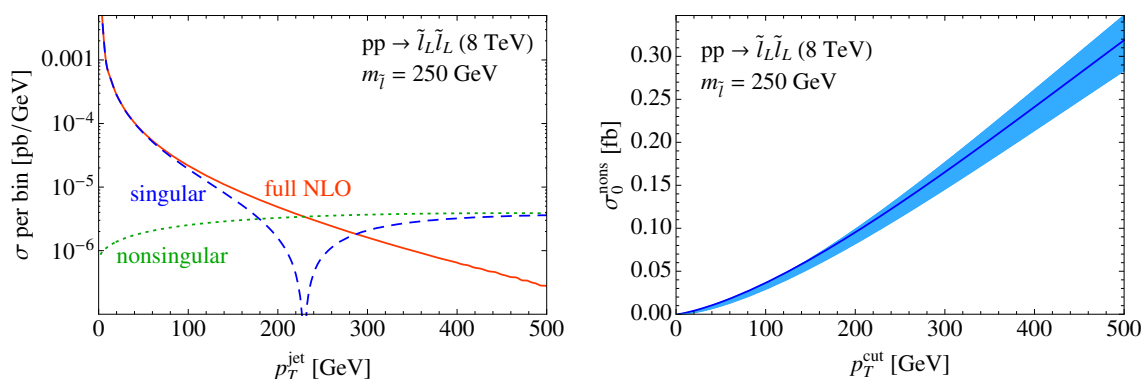
Figure 11. Left: singular (blue dashed) and nonsingular (green dotted) contributions to the full NLO (red solid) differential cross section for \tilde{\ell}_L\tilde{\ell}_L production. Right: the (integrated) nonsingular cross section for \tilde{\ell}_L\tilde{\ell}_L at NLO.
