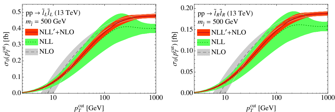
Figure 8. The 0-jet cross section for \tilde{\ell}_L\tilde{\ell}_L (left) and \tilde{\ell}_R\tilde{\ell}_R (right) production as a function of p_T^{\text{cut}} for m_{\tilde{\ell}} = 500 GeV at 13 TeV. The bands show the perturbative uncertainties.
