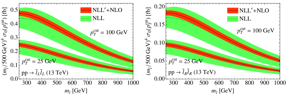
Figure 9. The 0-jet cross section for \tilde{\ell}_L\tilde{\ell}_L (left) and \tilde{\ell}_R\tilde{\ell}_R (right) production as a function of m_{\tilde{\ell}} for p_T^{\text{cut}} = 25 GeV and 100 GeV at 13 TeV. Shown are the NLL (green band, dotted line) and NLL'+NLO (red band, solid line) predictions with their perturbative uncertainty. We multiply the cross section by (m_{\tilde{\ell}}/500 \text{ GeV})^4 for better visibility.
