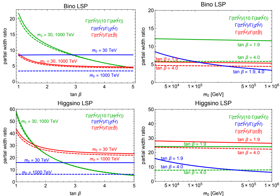
Figure 4. Gluino branching ratios, plotted as functions of a universal scalar mass scale m_0 and \tan\beta . We choose two benchmark points, both with M_3 = 2\text{ TeV} : in the top row, M_1 = 200\text{ GeV} , M_2 = 400\text{ GeV} , and \mu = 800\text{ GeV} ; in the bottom row, M_1 = 700\text{ GeV} , M_2 = 1\text{ TeV} , and \mu = 200\text{ GeV} . Because the b\bar{b} width is very small, we have multiplied it by 10 to make the green curves visible in the plot.
