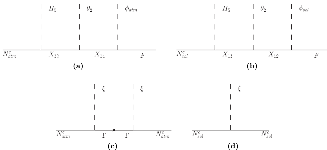
Figure 3. Renormalisable diagrams leading to neutrino effective terms. Diagrams (a) and (b) are responsible for neutrino Yukawa terms (leading to Dirac masses) while (c) and (d) give right-handed neutrino Majorana mass terms.
