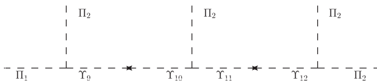
Figure 5. Diagram for non-renormalisable term in the 75 potential.
