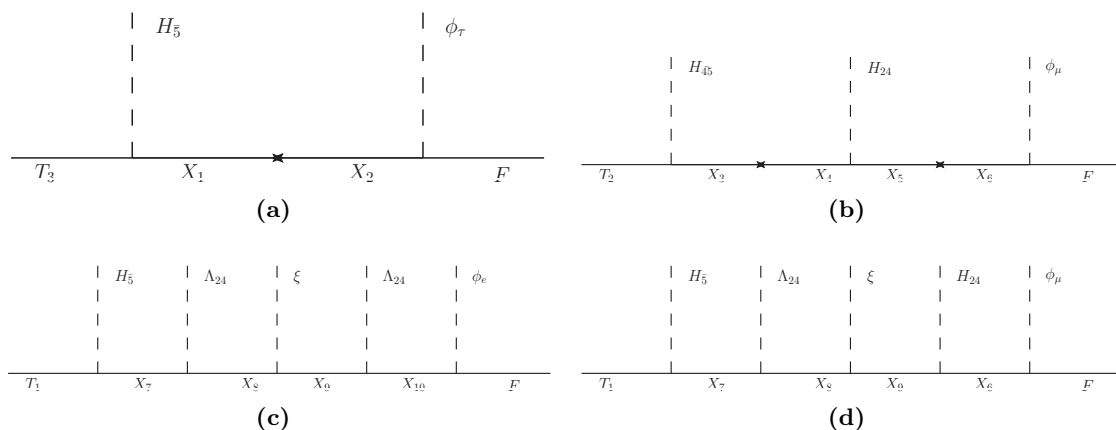
Figure 2. Diagrams responsible for the masses of the down-type quarks and charged leptons.
