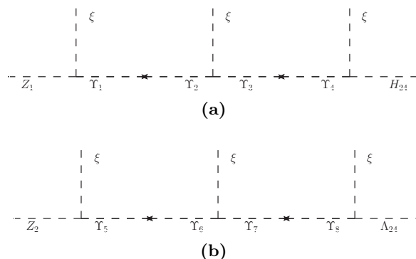
Figure 4. Diagrams for non-renormalisable potential terms.
