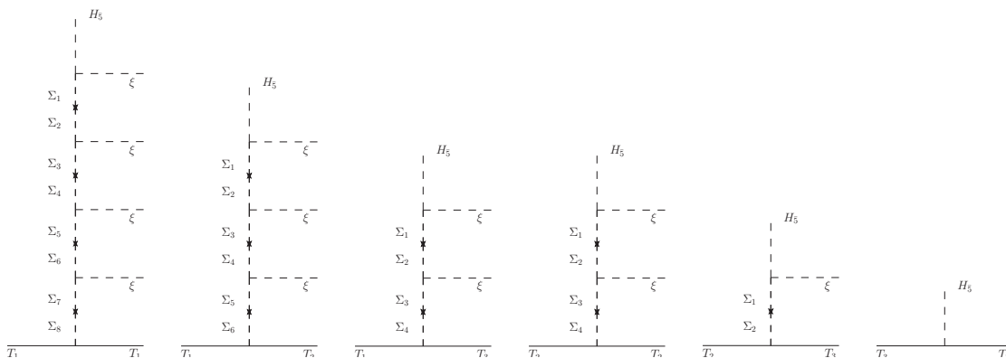
Figure 1. Diagrams responsible for the masses and mixings of the up-type quarks.
