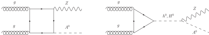
Figure 11. Representative Feynman diagrams for Z A^0 production in gluon fusion in the 2HDM.
