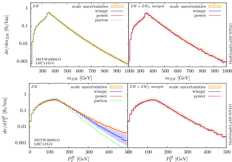
Figure 8. Invariant ZH mass and p_T^H distributions for gluon induced ZH production at \sqrt{s} = 14 TeV. The left column shows the results obtained for the gg \rightarrow ZH case, with different starting scale for the shower: “wimpy” and “power” shower. The blue band shows the variation of the shower scale for “wimpy” shower in the range 0.5\mu_F < Q_{PS} < 2\mu_F , while the yellow bands show the uncertainty associated with a factor of two variation of the renormalisation and factorisation scales with respect to their central value. The right column shows the same results for the merged sample. The green curves in the left column correspond to the parton level results before passing them through PYTHIA 8.
