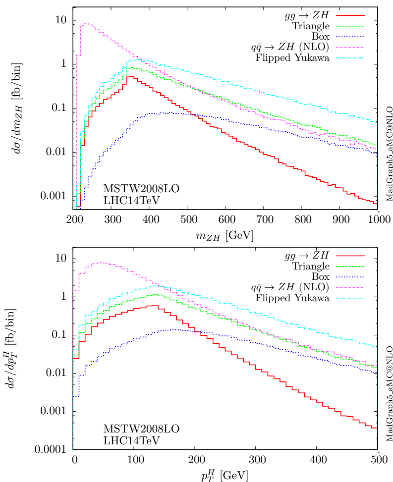
Figure 5. Invariant ZH mass and p_T^H distributions for ZH production at \sqrt{s} = 14 \text{ TeV} . The gluon fusion contribution is decomposed into the triangle and box contribution. For completeness we also plot the Drell-Yan type contributions at NLO obtained with MADGRAPH5_AMC@NLO .
