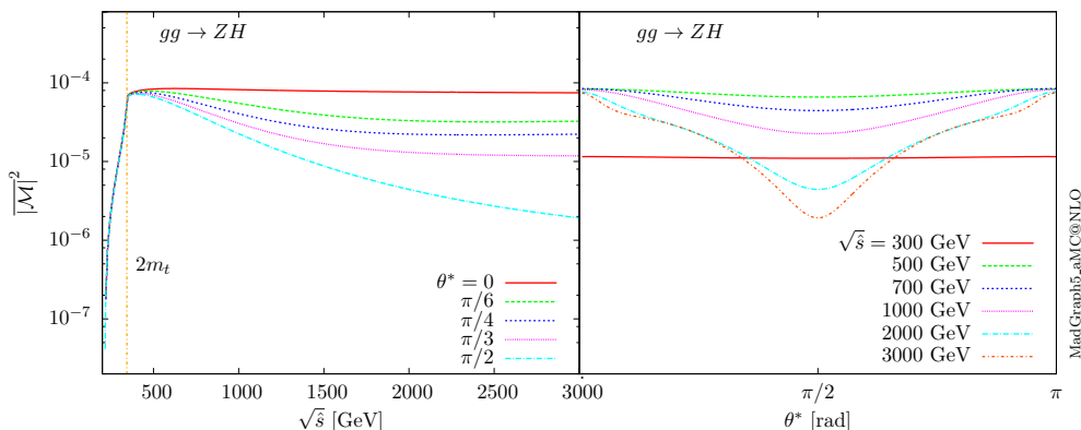
Figure 4. Matrix element squared for gg \rightarrow ZH as a function of the centre-of-mass energy for different values of scattering angles (left) and as a function of the centre-of-mass scattering angle for various values of \sqrt{\hat{s}} (right).
