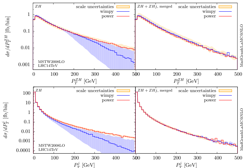
Figure 9. Transverse momentum of the ZH system and hardest jet p_T distributions for ZH production at \sqrt{s} = 14 TeV. The setup is the same as in figure 8.
