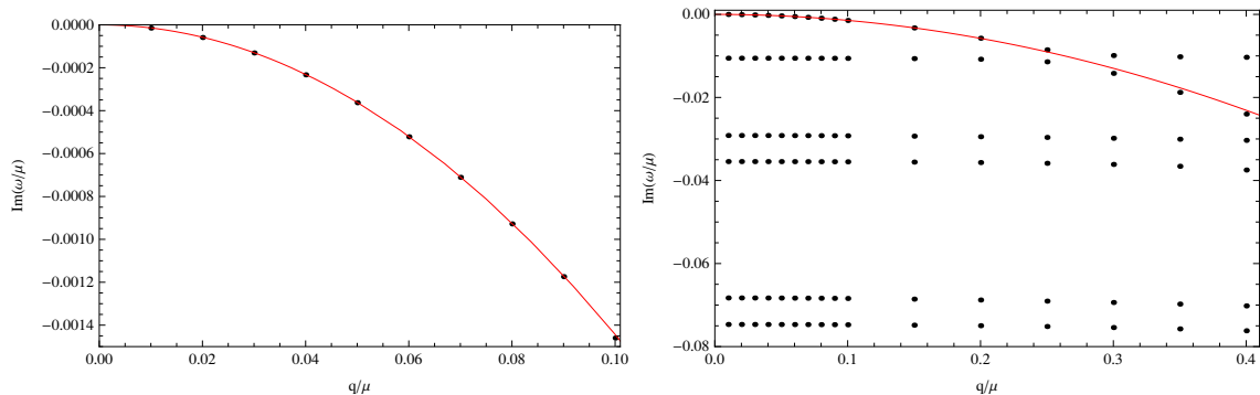
Figure 2. Dispersion relations of the purely imaginary ‘poles’ nearest the origin as determined by Leaver’s method, at fixed N_{\max.} = 300 (shown as dots). The red line shows the analytic result (4.12) for the T = 0 diffusion mode. The data on both plots is the same — the left hand plot is a magnified version of the near-origin region of the right hand plot.
