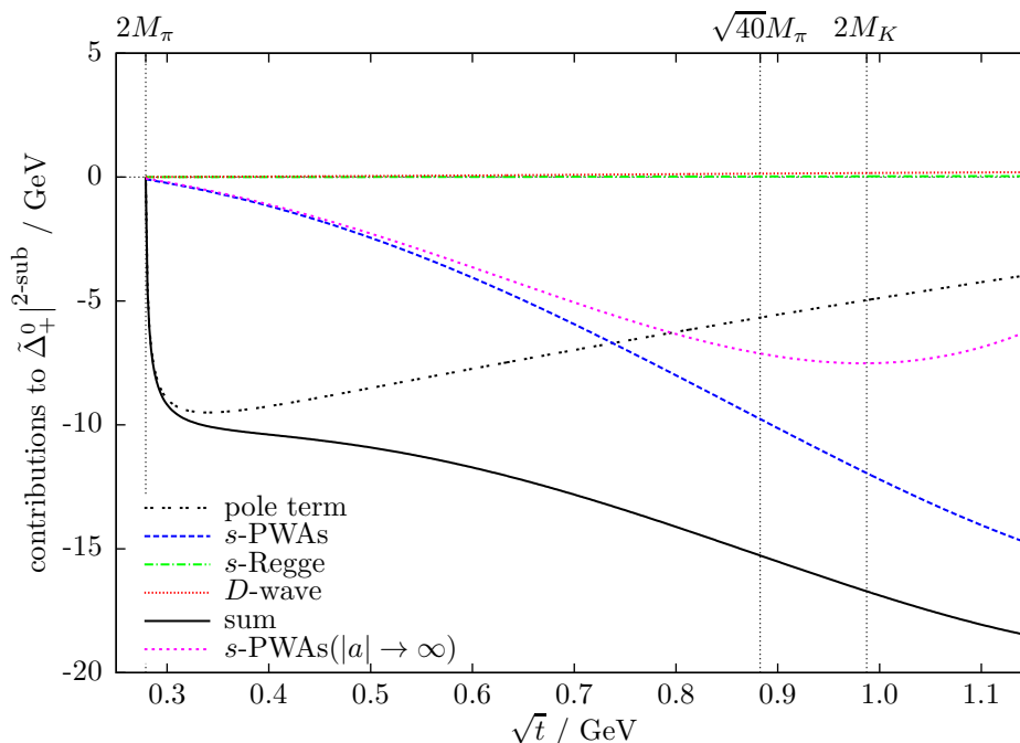
Figure 7. Contributions to the twice-subtracted S -wave MO inhomogeneity \tilde{\Delta}_+^0 |^{2-sub} .
