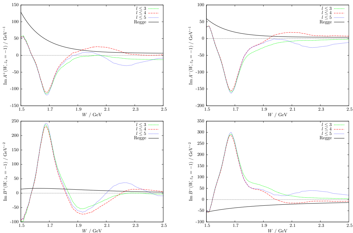
Figure 4. Matching of the s -channel absorptive parts between KH80 partial-wave contributions for l \leq 3 , l \leq 4 , and l \leq 5 and the \pi N backward scattering Regge model [73].
