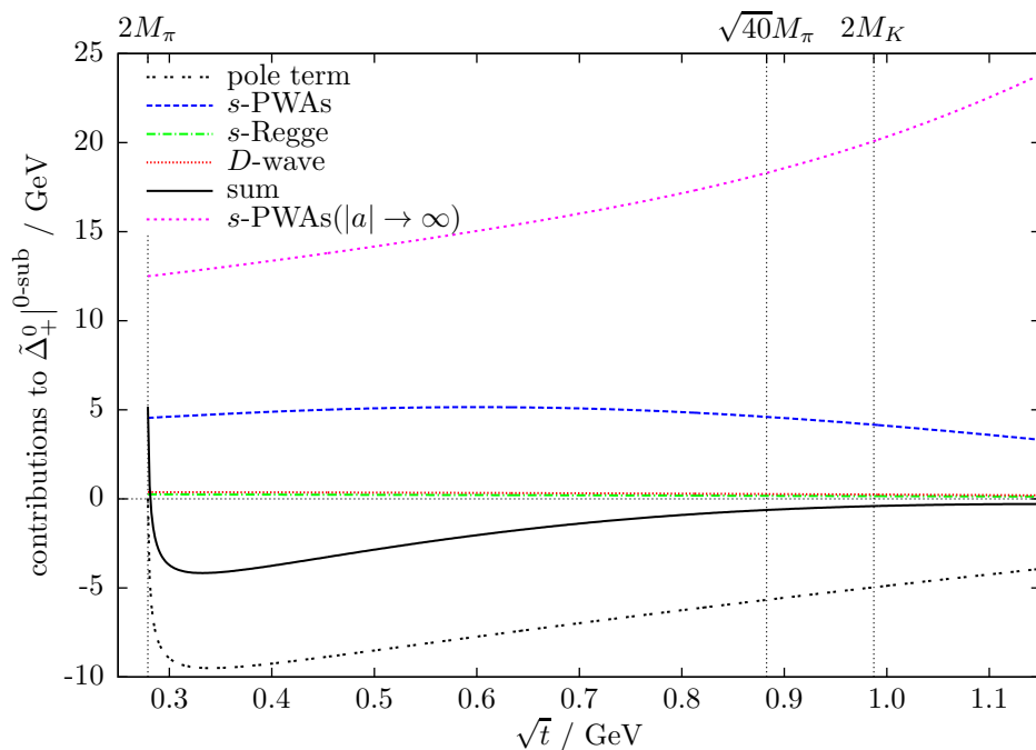
Figure 5. Contributions to the unsubtracted S -wave MO inhomogeneity \tilde{\Delta}_+^0|^{0-sub} . See text for details.
