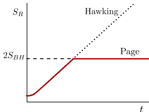
Figure 5. Page curve for the entropy of the radiation, for the model in figure 3. The dotted line is the growing result given by the Hawking computation, and the entropy calculated from the other saddle is dashed. The minimum of the two is the Page curve for this model.
