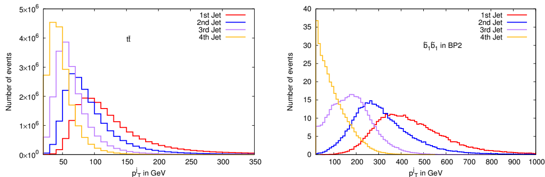
Figure 1. Ordered p_T^{\text{jet}} distribution for t\bar{t} (left) and for \tilde{b}_1\tilde{b}_1^* in BP2 (right) at an integrated luminosity of 50 \text{ fb}^{-1} .
