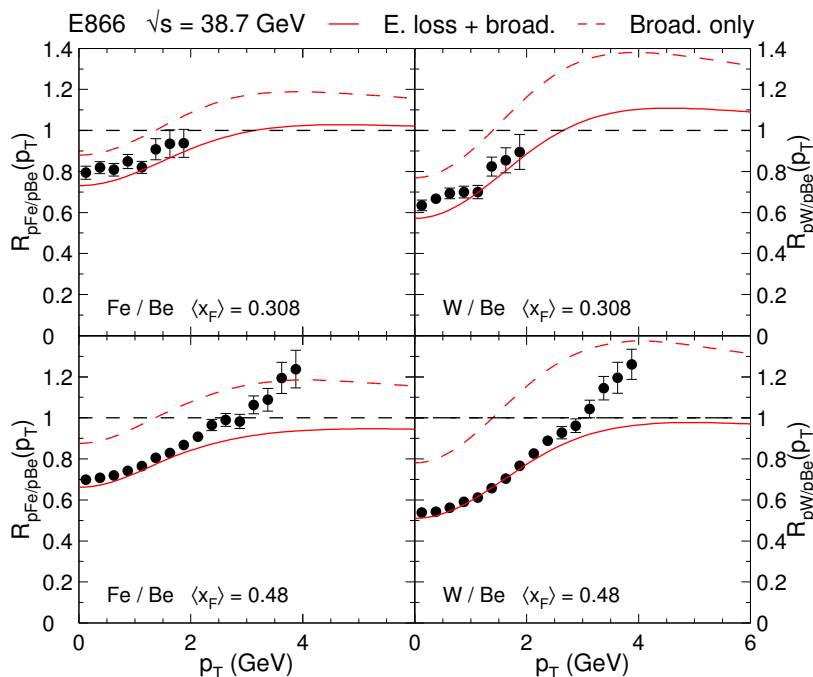
Figure 2. Model predictions (solid red curves) for the J/\psi nuclear suppression factor compared to the E866 data for R_{\text{Fe/Be}}(p_{\perp}) (left) and R_{\text{W/Be}}(p_{\perp}) (right), in the intermediate- x_F ( \langle x_F \rangle = 0.308 , top) and large- x_F ( \langle x_F \rangle = 0.48 , bottom) ranges. The dashed lines indicate the effect of momentum broadening only, R_{\text{pA}}^{\text{broad}}(y, p_{\perp}) , eq. (2.14).
