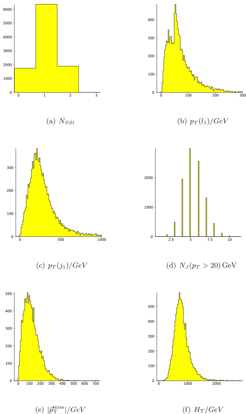
Figure 7. Distributions of quantities of interest for our test point m_{\tilde{g}} = 588 GeV, m_{\tilde{t}_1} = 581 GeV, for supersymmetric signal events. In (a), we show the number of isolated leptons passing minimum p_T cuts (where, if there are two, they must have the same sign). We use the CMS analysis' lepton isolation criteria. In (b), we show the hardest isolated lepton's p_T . Otherwise, the only cuts are that jets have p_T > 20 GeV, and jets and leptons lie within the fiducial region of the detector. Other detector effects are not taken into account.
