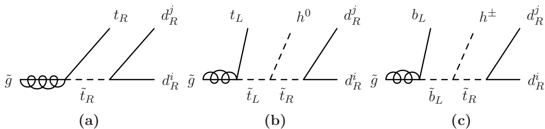
Figure 1. Gluino decays without right-handed bottom squarks in the presence of W \supset U_3 D_i D_j , via (a) right-handed top, (b) left-handed top, and (c) left-handed bottom. Same sign leptons are obtained in (c) only if the charged Higgs subsequently decays to t\bar{b} or to leptons.
