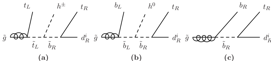
Figure 2. Gluino decays with right-handed bottom squarks in the presence of W \supset U_3 D_i D_3 , via (a) left-handed top squark, (b) left-handed bottom squark, and (c) right-handed bottom squark.
