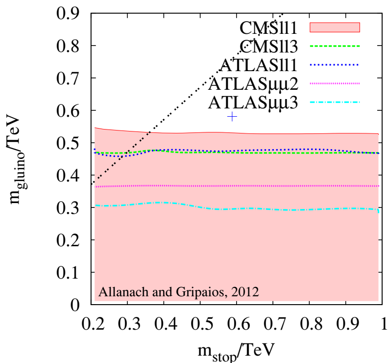
Figure 5. 95% exclusions from the CMS di-leptons \bar{p}_T^{\text{miss}} search (CMSII1,3), the ATLAS di-leptons \bar{p}_T^{\text{miss}} search (ATLASII1) and the ATLAS same-sign di-muons search (ATLAS \mu\mu 2,3). The signal regions of each analysis, corresponding to the number are defined in tables 2, 3, 4. The cross shows the location of our test point. We have not combined the different exclusion regions, but have merely shaded the area excluded by the most constraining search. Above and to the left of the black dashed diagonal line, gluino decays are through on-shell stops, whereas underneath and to the right of it, gluino decays are through off-shell stops.
