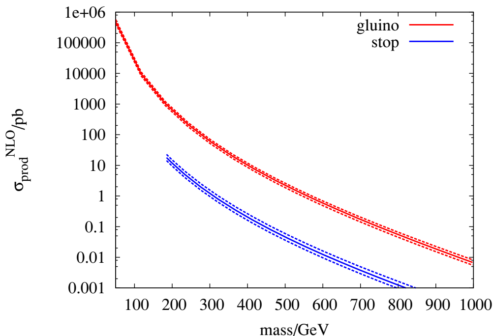
Figure 3. Stop and gluino total production cross-sections at a 7 TeV LHC calculated at NLO by PROSPINO2.1. The dashed curves show the variations due to changes in the renormalisation scale by a factor of two.
