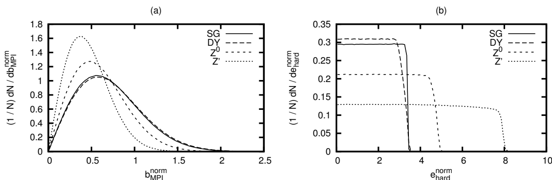
Figure 5. Low-mass Drell-Yan, Z^0 and Z' production in pp collisions at \sqrt{s} = 7 TeV. (a) The impact parameter distribution and (b) enhancement factor of the hard interaction per event. The single Gaussian distributions are identical between the three processes
