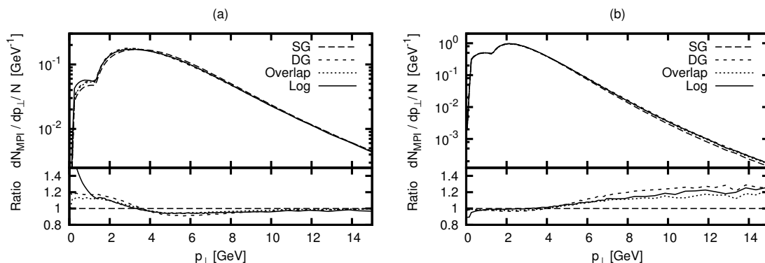
Figure 9. p_{\perp} distribution (a) of the hard process and (b) inclusive for subsequent MPI in minimum bias events. Ratio plots are normalised to the single Gaussian result
