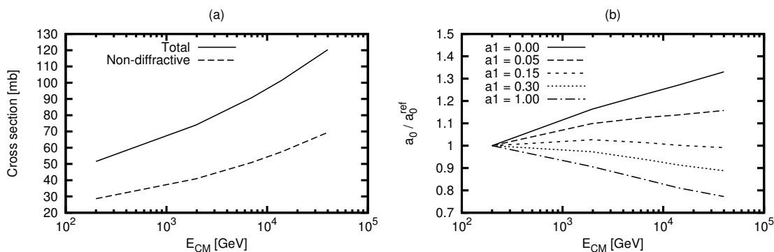
Figure 1. (a) The rise of the total and non-diffractive pp cross section with energy, and (b) the ratio a_0(E_{CM})/a_0(200 \text{ GeV}) , over the same energy range, for a set of different a_1 values
