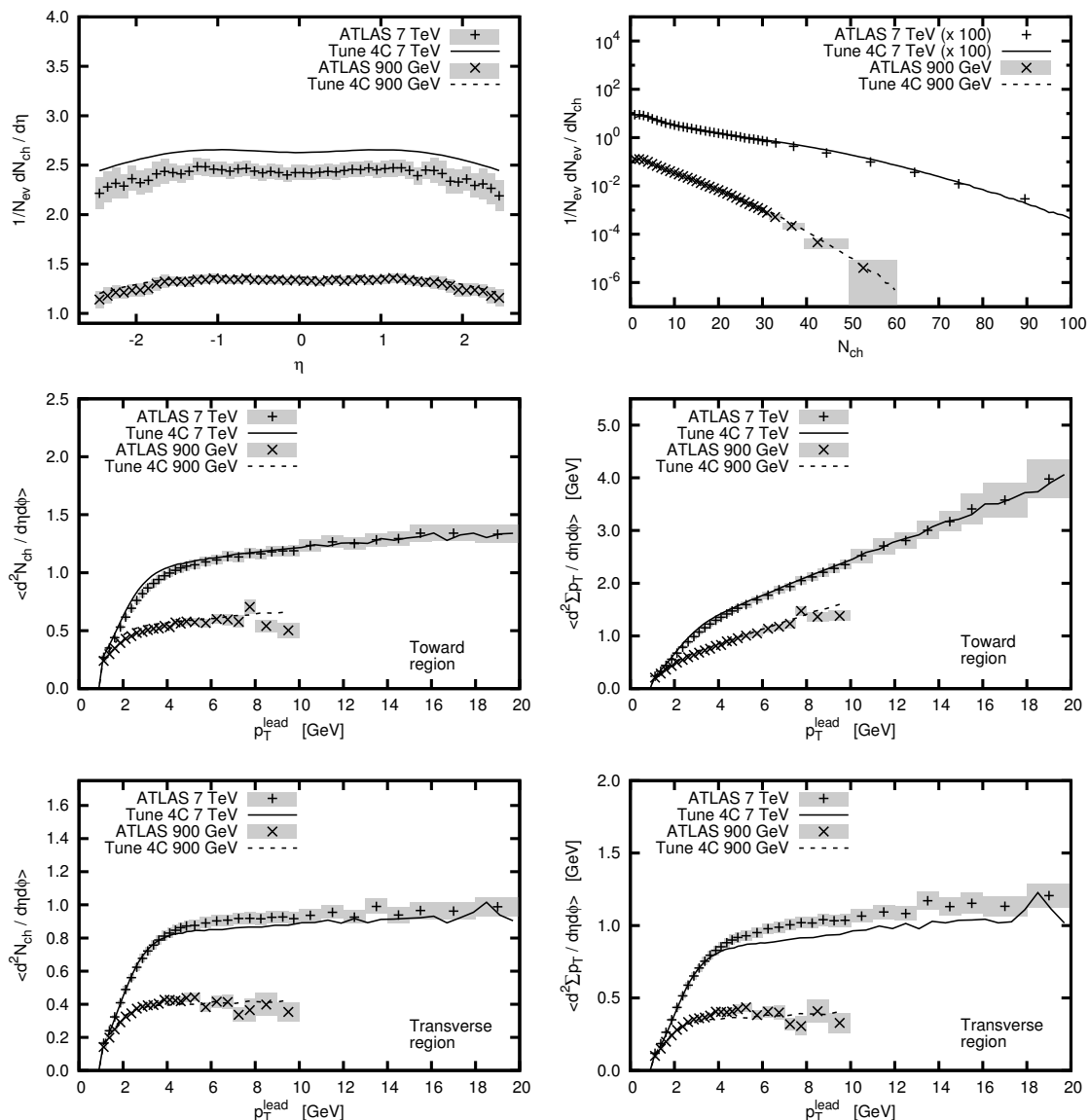
Figure 10. Tune 4C compared against early LHC data. Further details are given in the text
