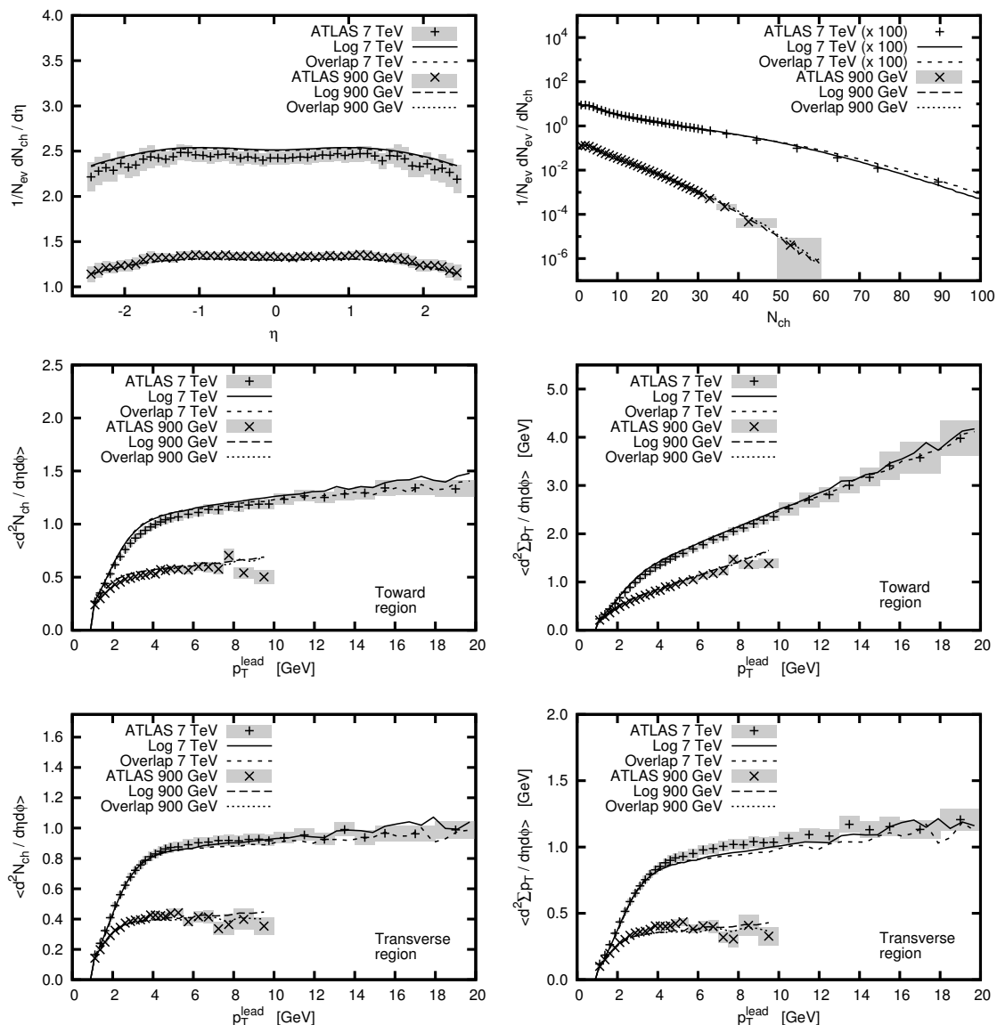
Figure 11. Tune 4C, using the log profile, and with a raised p_{\perp 0} in the MPI framework, compared against an overlap profile with p = 1.6 , also with a raised p_{\perp 0} , and LHC data
