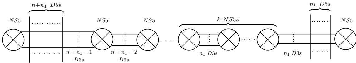
Figure 13. The brane construction after brane moves of S_f \cap X_M with f = [(n+k-1)^{n_1}, 1^{n+n_1}] and M = [(n+k)^{n_1}, n] .
