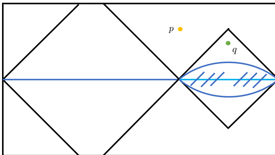
Figure 4. The regions D[R] and D[\bar{R}] for an asymmetric division of the system in the case of a boundary dS_2 spacetime, whose Penrose diagram we depict here. The region E[R] for R the smaller subregion is indicated by the dark blue hatchmarks. Operators at the point p can be causally influenced from either region and are not in \text{EW}[R] or \text{EW}[\bar{R}] ; this is familiar in asymptotic AdS/CFT. The point q illustrates a point in D[R] which is not in E[R] . Operators at that point do not commute with those in the algebra \mathcal{A}_{\bar{R}_s} corresponding to the complementary subsystem to R . We note that this point q on the boundary is also not part of the EW of either R or \bar{R} , since it can be reached causally from both.
