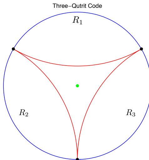
Figure 7. The Three-Qutrit Code example.
