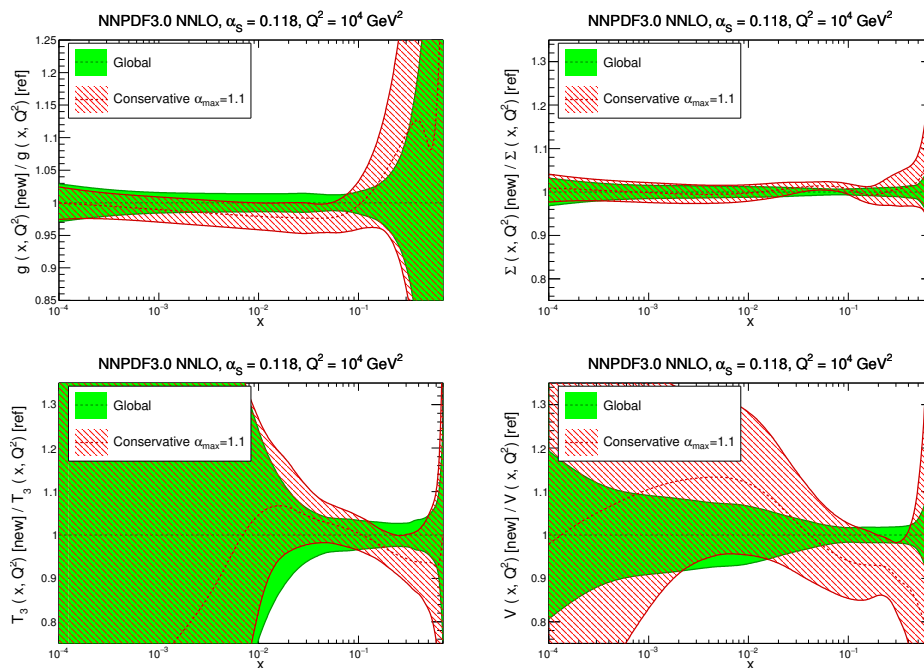
Figure 44. Same as figure 43, but at Q^2 = 10^4 \text{ GeV}^2 , and with results shown as ratios to the NNPDF3.0 default global fit.
