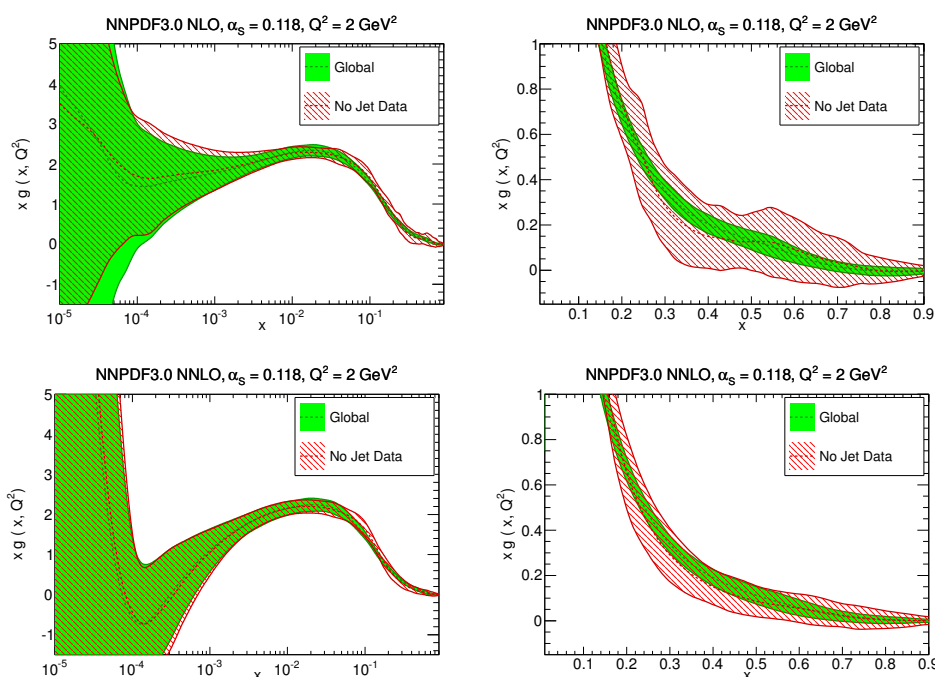
Figure 53. Comparison of the gluon in a fit to a dataset without jet data and in the global fit at NLO (top) and NNLO (bottom), plotted at Q^2 = 2 \text{ GeV}^2 vs. x on a logarithmic (left) and linear (right) scale.
