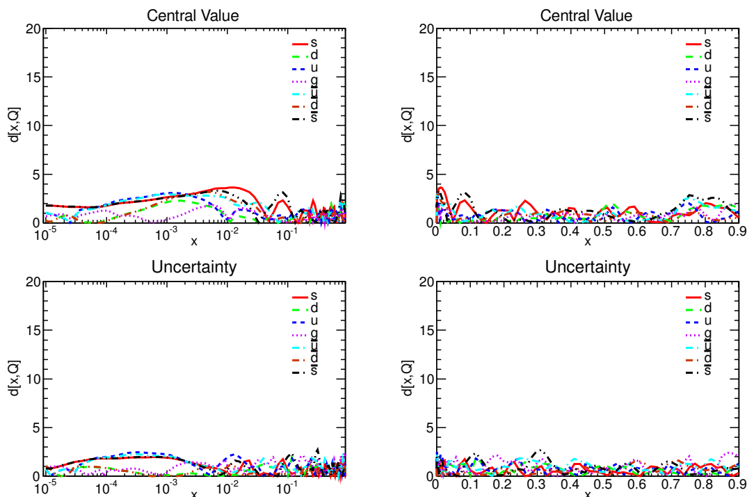
Figure 23. Same as figure 19 for the Level 2 closure fits based on the NNPDF3.0 and NNPDF2.3 input parametrization basis, fits C9 and C112 in table 8.
