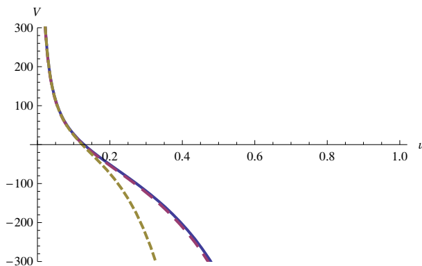
Figure 3. The potential barrier for the A_x gauge field. The infinite 't Hooft coupling limit is indicated by a solid line, while the dashed and dotted lines have \lambda = 50 . We have used r_q = 1.14 , \kappa_0 = 20 and \mathcal{K}_0 = 3\sqrt{3}/2 for all three curves. The dashed line only contains metric corrections while the dotted line includes both metric and the C^4 corrections of eq. (B.10).
