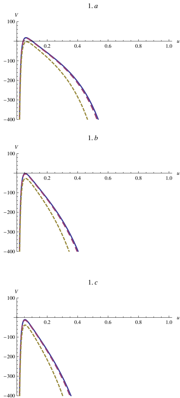
Figure 1. The potential barrier for the A_0 gauge field. In each figure there are three different values for the 't Hooft coupling, i.e. \lambda \rightarrow \infty , 50 and 10, indicated by solid, dashed and dotted lines, respectively. Figures 1.a, 1.b and 1.c correspond to different values of the parameters r_q and \kappa_0 . In figure 1.a r_q = 1.14 and \kappa_0 = 20 ; in figure 1.b r_q = 1.539 and \kappa_0 = 27 ; while in figure 1.c r_q = 1.71 and \kappa_0 = 30 . \mathcal{K}_0 has been set to 3\sqrt{3}/2 for all curves.
