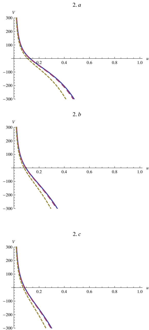
Figure 2. The potential barrier for the transverse modes A_i(u) . In each figure there are three different values for the 't Hooft coupling, i.e. \lambda \rightarrow \infty , 50 and 10, indicated by solid, dashed and dotted lines, respectively. Figures 2.a, 2.b and 2.c correspond to different values of the parameters r_q and \kappa_0 . In figure 2.a r_q = 1.14 and \kappa_0 = 20 ; in figure 2.b r_q = 1.539 and \kappa_0 = 27 ; while in figure 2.c r_q = 1.71 and \kappa_0 = 30 . \mathcal{K}_0 has been set to 3\sqrt{3}/2 for all curves.
