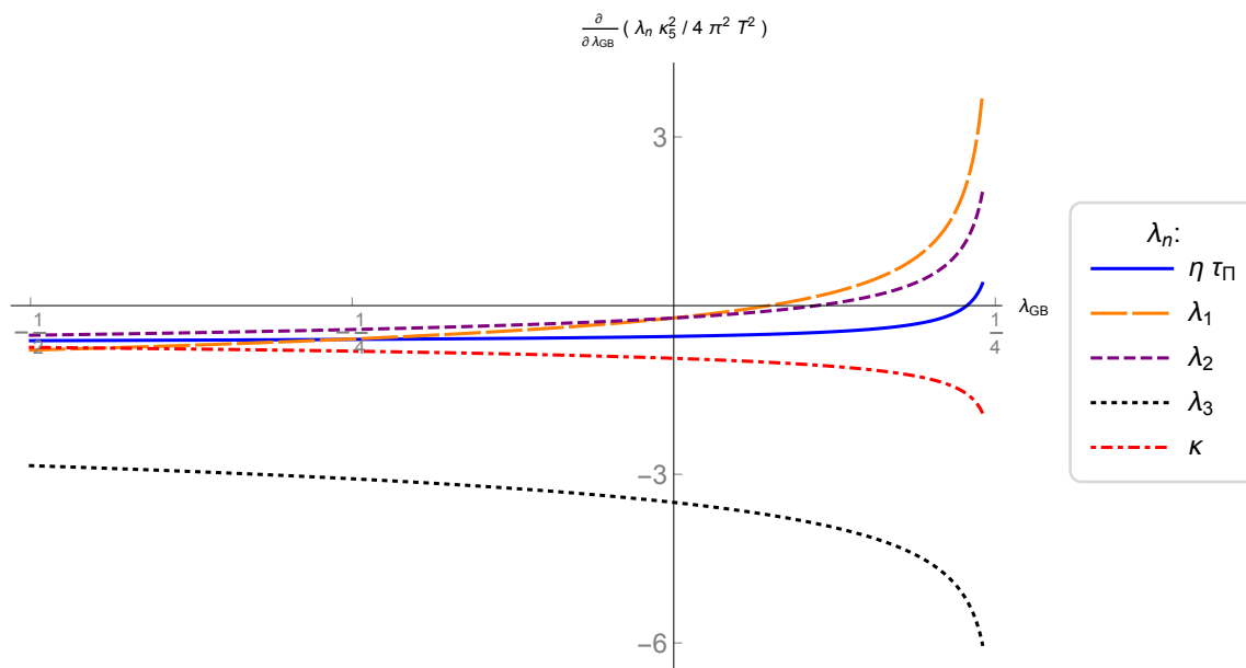
Figure 3. Derivatives of the second-order coefficients \lambda_n = \{\eta\tau_\Pi, \lambda_1, \lambda_2, \lambda_3, \kappa\} with respect to \lambda_{\text{GB}} , in units of 4\pi^2 T^2/\kappa_5^2 , as functions of \lambda_{\text{GB}} .
