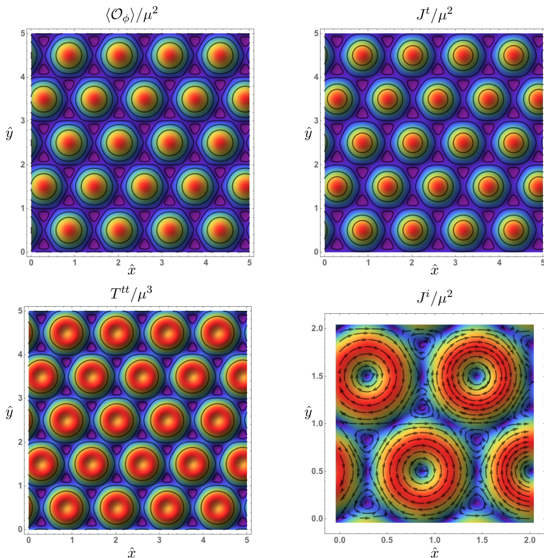
Figure 4. The spatial behaviour of various expectation values for the thermodynamically preferred triangular lattice at T/\mu = 0.04 . Top left shows the expectation value of the pseudo scalar operator \langle \mathcal{O}_\phi \rangle / \mu^2 , top right shows the charge density J^t / \mu^2 , bottom left shows T^{tt} / \mu^3 and bottom right shows the flow lines and the norm of the magnetisation currents J^i / \mu^2 . The plots are functions of the spatial coordinates (\hat{x}, \hat{y}) \equiv (\frac{x'}{L_x}, \frac{y'}{L_y}) and colours with longer wavelength correspond to larger values (the norm of J^i / \mu^2 for the bottom right).
