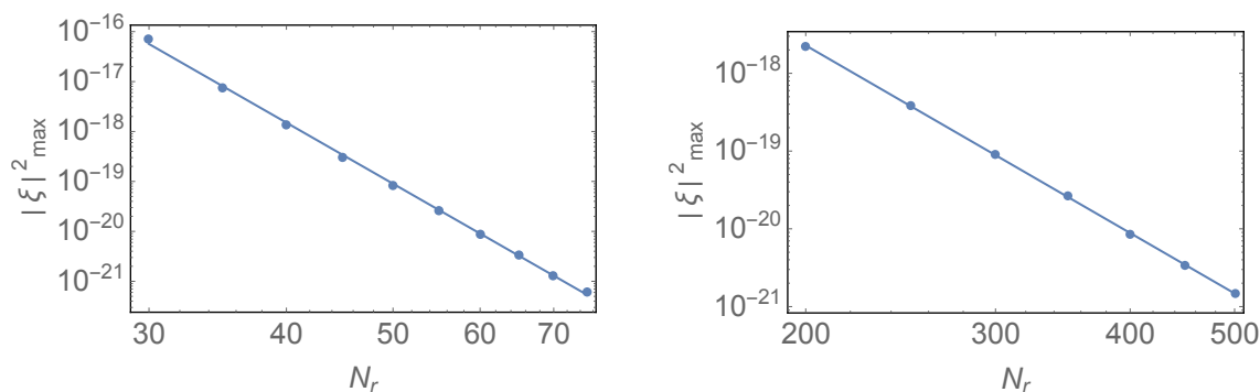
Figure 6. Convergence plots of the maximum value of |\xi|_{\max}^2 in our computational grid as a function of grid points in the radial direction r for Chebyshev spectral (left) and fourth order finite differences (right). Both plots are for T/\mu = 0.05 , k_x = k_y = 0.97 \mu , R_0 = 0 and B = 0.05 \mu^2 .
