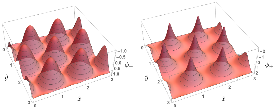
Figure 5. A plot of the spatial dependence of the scalar field on the black hole horizon, \phi_+ \equiv \phi(r_+) , as a function of the spatial coordinates (\hat{x}, \hat{y}) \equiv (\frac{x'}{L_x}, \frac{y'}{L_y}) . The left plot is for the thermodynamically preferred triangular lattice at T/\mu = 0.04 . The right plot is for the preferred triangular lattice at T/\mu = 0.01 .
