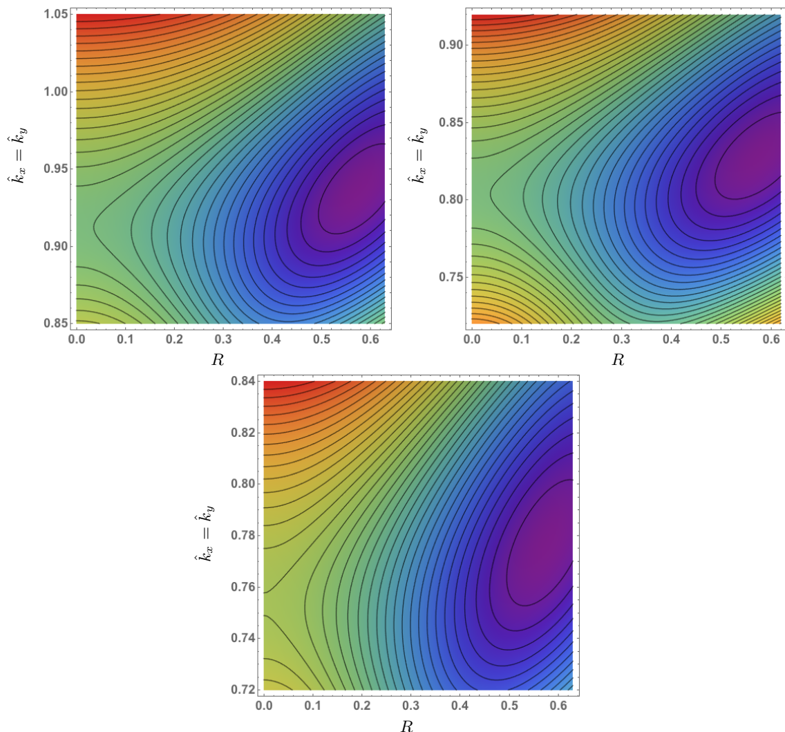
Figure 2. Free energy of the rhombiboard lattices. The contours display the free energy density \hat{w} \equiv w/\mu^3 as a function of R_0 and \hat{k}_x = \hat{k}_y , where \hat{k}_x \equiv k_x/\mu and \hat{k}_y = k_y/\mu , for temperatures T/\mu = 0.07 (top left), T/\mu = 0.05 (top right) and T/\mu = 0.04 (bottom). Colours with longer wavelength correspond to contours with larger values. The minimum is at R_0 = 1/\sqrt{3} , corresponding to triangular lattices, in all three cases but the period changes with temperature. The minima for the three cases are located at \hat{k}_x = 0.937 , \hat{k}_x = 0.828 and \hat{k}_x = 0.777 , respectively.
