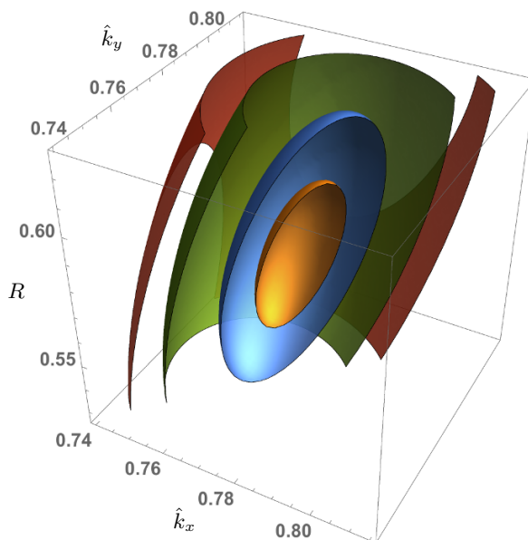
Figure 3. Surfaces of constant free energy density \hat{w} \equiv w/\mu^3 in the three dimensional module space (\hat{k}_x, \hat{k}_y, R_0) , where \hat{k}_x \equiv k_x/\mu and \hat{k}_y = k_y/\mu . The plot was made for the T/\mu = 0.04 case of figure 2. The minimum is for the triangular lattice with R = 1/\sqrt{3} and equal periods \hat{k}_x = \hat{k}_y = 0.777 .
