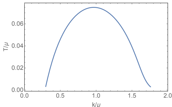
Figure 1. For black holes in the unbroken phase with B/\mu^2 = 0.05 we plot the critical temperature, T_c , for the onset of a striped instability with wave number k . The bulk model is as in (2.9) with (s, \chi) = (1, 1.5) . The maximum temperature for which we find a zero mode is at T/\mu = 0.075 with k/\mu = 0.967 .
