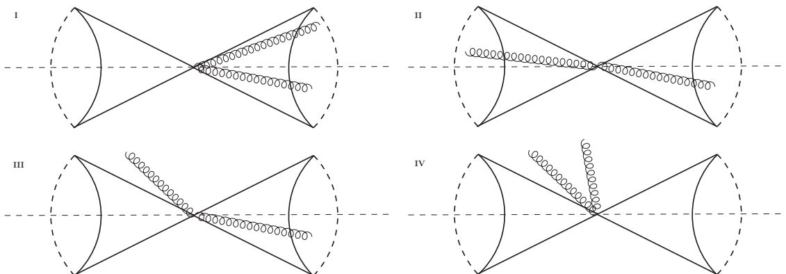
Figure 3. Final state phase space configurations containing two soft partons. Panel I shows two soft gluons going into the right jet, panel II shows one soft gluon going into the right jet and another going into the left jet, panel III shows one soft gluon going into the right jet and one soft gluon going out of all jets, and, finally, panel IV shows two soft gluons going out of all jets. In the above, it is in all cases possible to replace the two soft gluons with a soft quark-antiquark pair.
