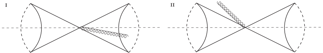
Figure 2. Final state phase space configurations with a single soft parton. Panel I shows a single soft gluon going into the right jet and panel II shows a single soft gluon going out of all jets.
