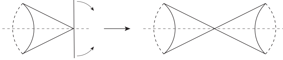
Figure 4. A hemisphere boundary can be mapped onto a cone boundary by choosing an appropriate Lorentz boost.
