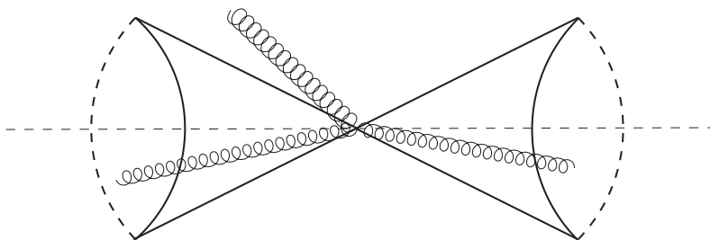
Figure 5. Starting at \mathcal{O}(\alpha_s^3) , there will be contributions to the \tau_\omega soft function which simultaneously probe all three regions of the final state phase space.
