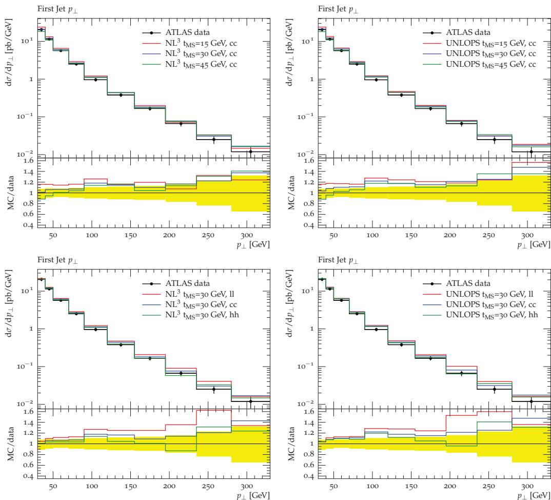
Figure 10. Transverse momentum of the hardest jet in W-boson production, as measured by ATLAS [47]. The MC results were obtained by merging up to two additional partons at LO, and zero and one additional parton at NLO. MC results are shown for three different t_{MS} merging scales (top panels) and for three different renormalisation/factorisation scales (bottom panels). Effects of multiple scatterings and hadronisation are included. Left panels: results of NL 3 . Right panels: results of UNLOPS.
