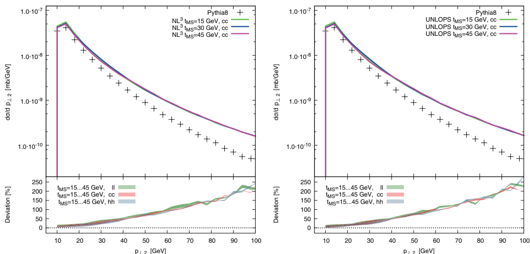
Figure 5. Transverse momentum of the second hardest jet, for W-boson production in pp collisions at E_{\text{CM}} = 7000 GeV, when merging up to two additional partons at LO, and zero and one additional parton at NLO. Jets were defined with the k_{\perp} -algorithm, with k_{\perp, \text{min}} = 10 GeV. Multi-parton interactions and hadronisation were excluded. The lower inset shows the deviation from PYTHIA8. Left panel: results of NL 3 . Right panel: results of UNLOPS.
