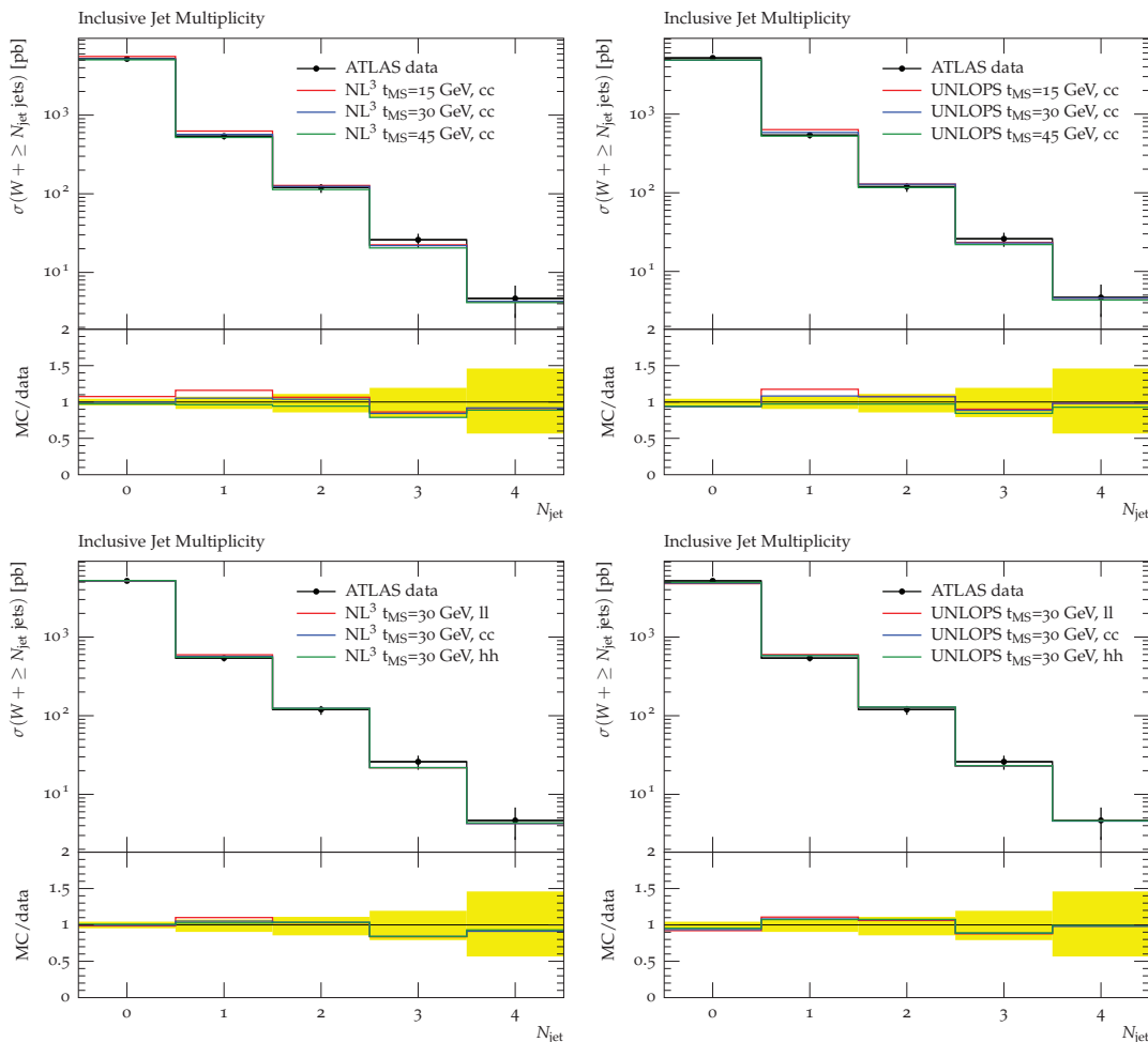
Figure 9. Jet multiplicity in W-boson production, as measured by ATLAS [47]. The MC results were obtained by merging up to two additional partons at LO, and zero and one additional parton at NLO. MC results are shown for three different merging scales (top panels) and for three different renormalisation/factorisation scales (bottom panels). Effects of multiple scatterings and hadronisation are included. Left panels: results of NL 3 . Right panels: results of UNLOPS.
