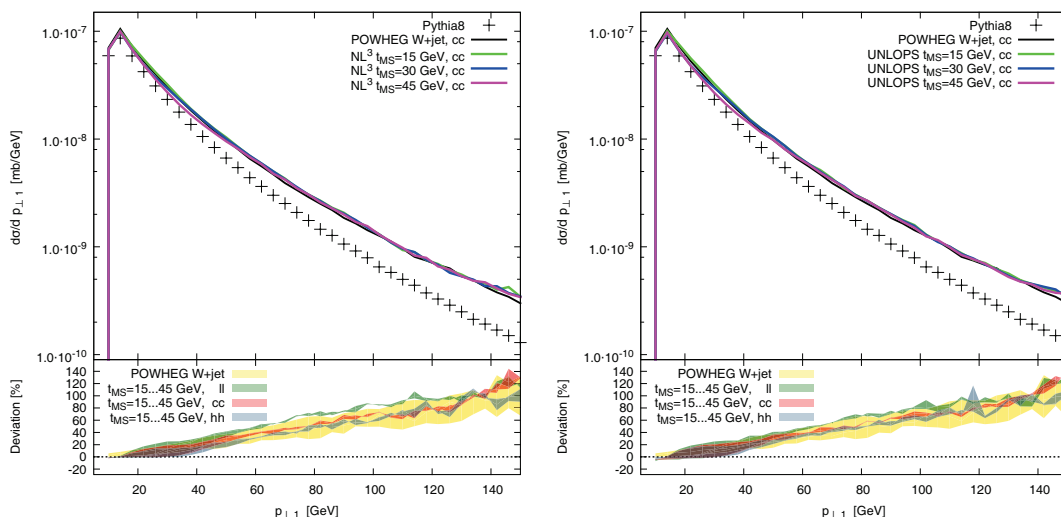
Figure 4. Transverse momentum of the hardest jet, for W-boson production in pp collisions at E_{\text{CM}} = 7000 GeV, when merging up to two additional partons at LO, and zero and one additional parton at NLO. Jets were defined with the k_{\perp} -algorithm, with k_{\perp, \text{min}} = 10 GeV. Multi-parton interactions and hadronisation were excluded. The lower inset shows the deviation from PYTHIA8. The band labelled “POWHEG W+jet” is given by the envelope of varying the renormalisation scale in the POWHEG-BOX program between \frac{1}{2}M_Z, \dots, 2M_Z , and the factorisation scale between \frac{1}{2}M_W, \dots, 2M_W . Left panel: results of NL 3 . Right panel: results of UNLOPS.
