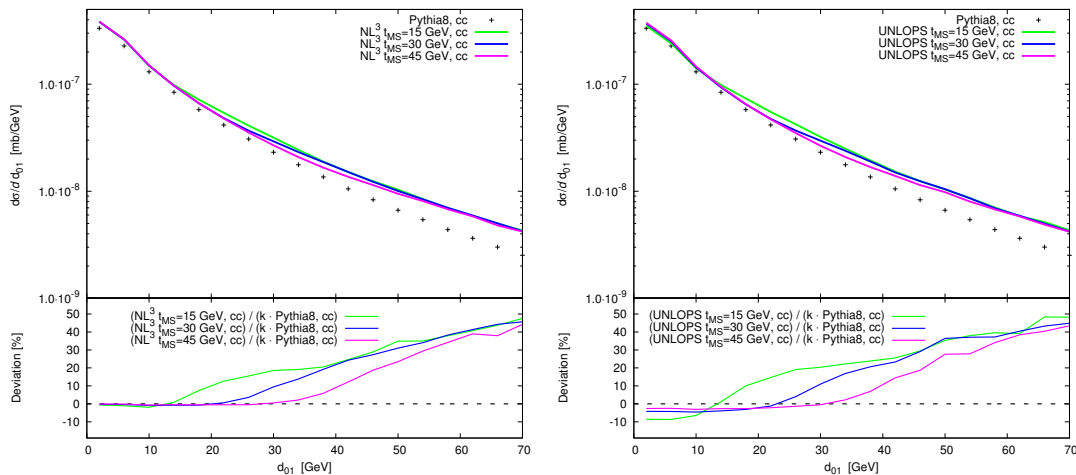
Figure 2. k_{\perp} - separation d_{01} of the first jet and the beam, for W-boson production in pp collisions at E_{CM} = 7000 GeV, when merging up to two additional partons at LO, and zero and one additional parton at NLO, for three different merging scales. Jets were defined with the k_{\perp} -algorithm, by clustering to exactly one jet. Multi-parton interactions and hadronisation were excluded. Left panel: results of the NL^3 scheme. Right panel: results of the UNLOPS scheme.
