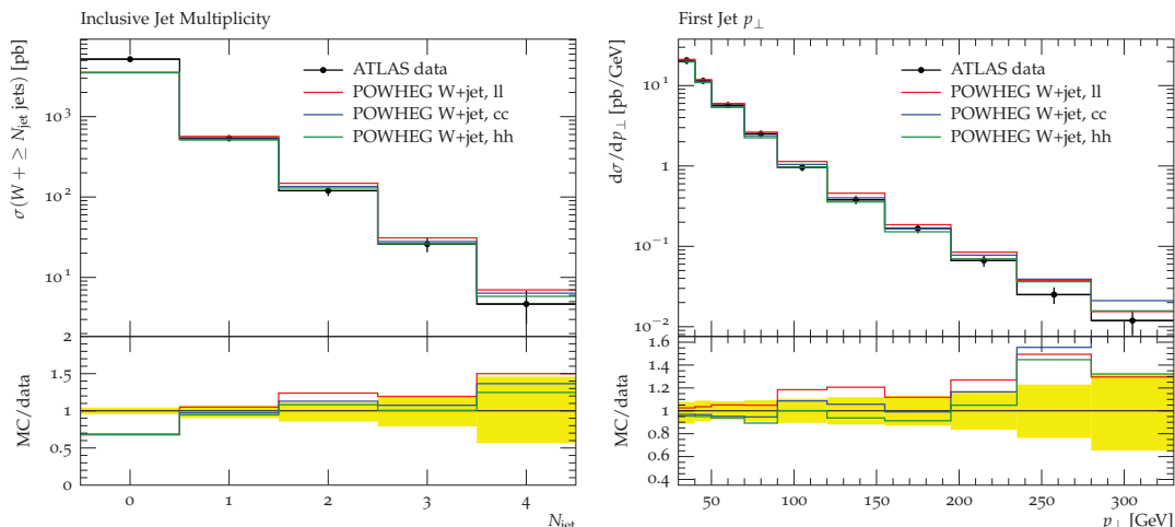
Figure 8. Jet multiplicity and transverse momentum of the hardest jet in W-boson production, as measured by ATLAS [47]. MC results taken from the POWHEG-BOX program, with three different renormalisation/factorisation scales. Effects of partons showers, multiple scatterings and hadronisation are included.
