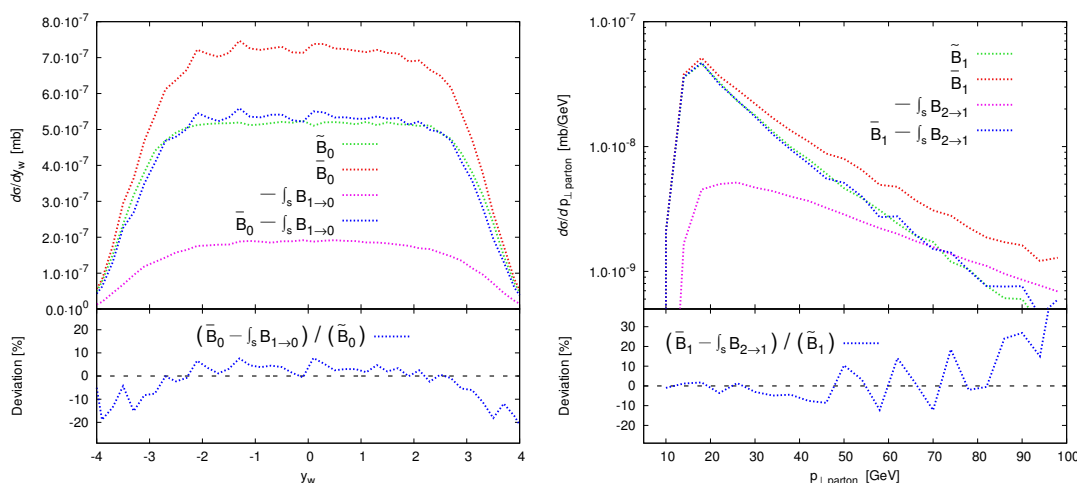
Figure 11. Comparisons of two ways of generating exclusive NLO cross sections. \bar{B}_i events are calculated without changing the POWHEG-BOX program, while for \tilde{B}_i , we have explicitly introduced the necessary cuts in POWHEG-BOX. Left panel: comparison for zero-jet exclusive NLO cross section, as function of the W-boson rapidity. Right panel: comparison for one-jet exclusive NLO cross section, as function the kinematical transverse momentum of the parton.
