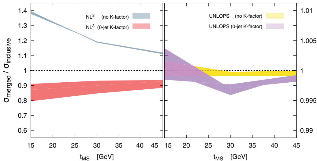
Figure 7. Comparison of inclusive cross sections for H-production in gluon fusion pp collisions at E_{\text{CM}} = 7000 \text{ GeV} , for \text{NL}^3 (left panel) and UNLOPS (right panel), when merging up to two additional partons at LO, and zero and one additional parton at NLO. The results of the merging procedure (labelled \sigma_{\text{merged}} ) are normalised to the zero-jet inclusive NLO cross section \sigma_{\text{inclusive}} . The coloured bands indicate the variation from choosing \mu_F in [(\frac{1}{2}M_H)^2, \dots, (2M_H)^2] and \mu_R in [(\frac{1}{2}M_Z)^2, \dots, (2M_Z)^2] . The results of the NLO merging procedure are presented for two different K -factor treatments. The result of using no K -factor is labelled “no K -factor”. Usage of the zero-jet K -factor is indicated by the label “0-jet K -factor”. The same variations of \text{NL}^3 and UNLOPS are plotted, albeit with a smaller ordinate scale for UNLOPS.
