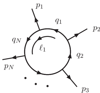
Figure 1. Momentum configuration of the one-loop N -point scalar integral.
