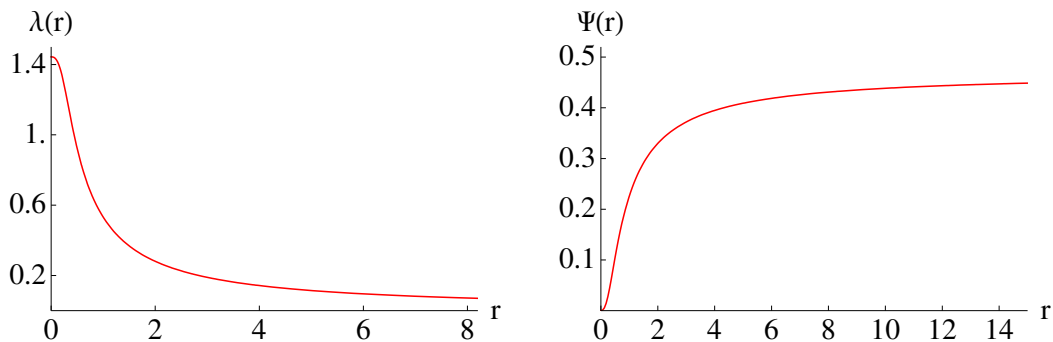
Figure 5. The scalar, \lambda , and the gauge field, \Psi , as functions of r for the T = 0 flow with \lambda_2 = 0 boundary condition.
