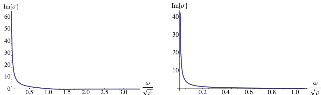
Figure 9. The imaginary part of the electric conductivity as a function of the frequency for the solutions with \lambda_2 = 0 (left) and \lambda_1 = 0 (right) at T = 0 . It is clear that there is a pole at \omega = 0 .
