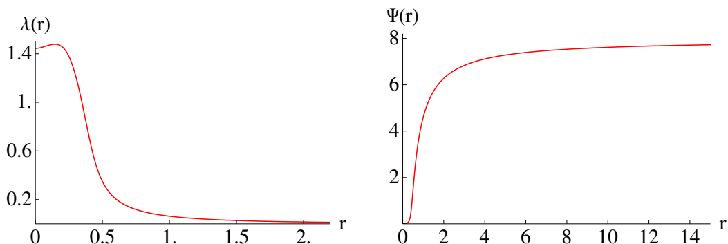
Figure 6. The scalar, \lambda , and the gauge field, \Psi , as functions of r for the T = 0 flow with \lambda_1 = 0 boundary condition.
