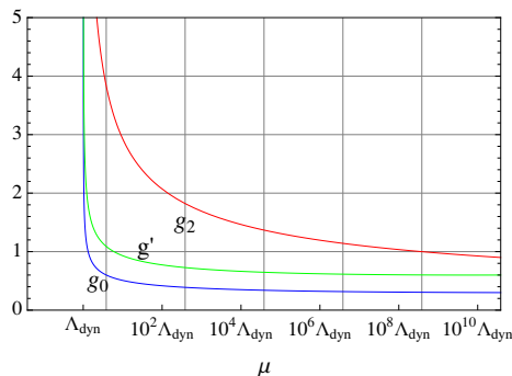
Figure 4. The running of the coupling constants under the renormalization group evolution. We have taken g_2(M_{\text{GUT}}) = 0.9 which leads to \Lambda_{\text{dyn}} = O(10^2) TeV. We have also taken g_0(M_{\text{GUT}}) = 0.3 and g'(M_{\text{GUT}}) = 0.6 . The figure shows that the Yukawa coupling constants become strong at the energy scale around \Lambda_{\text{dyn}} .
