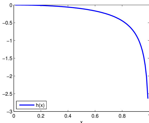
Figure 5. The function h(x) ( x = ke/2m^2 ) given in (C.3), which represents the size of the tachyonic mass in the model based on the D-term SUSY breaking. The value of |h(x)| is highly enhanced in the region x \rightarrow 1 , which corresponds to an IR singularities in the one-loop diagram.
