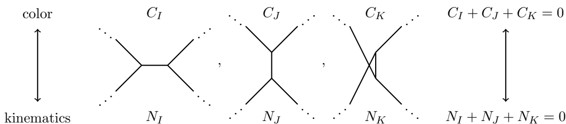
Figure 5. Triplets of cubic graphs I, J, K whose color factors C . and kinematic factors N . are both related by a Jacobi identity if the duality between color and kinematics is manifest. The dotted lines at the corners represent arbitrary tree-level subdiagrams and are understood to be the same for all of the three cubic graphs.
