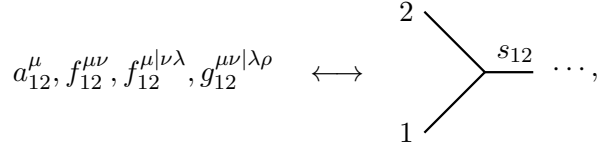
Figure 10. Diagrammatic interpretation of two-particle polarizations a_{12}^\mu, f_{12}^{\mu\nu}, f_{12}^{\mu|\nu\lambda}, g_{12}^{\mu\nu|\lambda\rho} .
