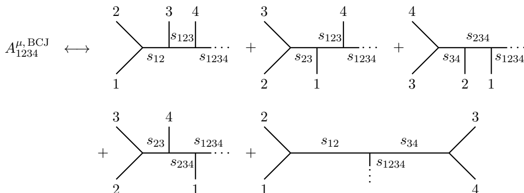
Figure 12. Cubic-diagram expansion of the rank-four Berends-Giele current A_{1234}^{\mu, BCJ} built from multiparticle polarizations.
