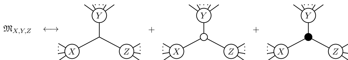
Figure 8. In the diagrammatic interpretation of the building block \mathfrak{M}_{X,Y,Z} in (3.15), the central vertex can either be of YM type (first term), of (\alpha'F^3) -type (white dot) or of (\alpha'^2F^4) -type (black dot). The blobs labelled by X, Y, Z represent currents of (\text{YM}+F^3+F^4) .
