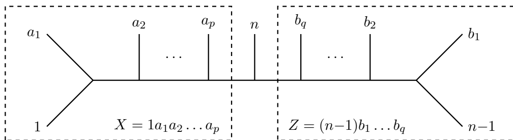
Figure 14. An alternative choice of master numerators composed of multiparticle polarizations of smaller rank as compared to (5.19). The external legs a_1, a_2, \dots, a_p, b_1, b_2, \dots, b_q are permutations of 2, 3, \dots, n-2 where p+q = n-3 and p = 0, 1, \dots, n-3 .
