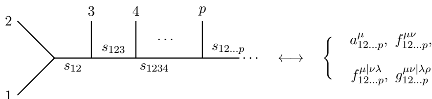
Figure 9. This section is dedicated to constructing local and Jacobi-satisfying kinematic representatives for the depicted cubic diagram of (YM+F^3+F^4) . The notation a_{12\dots p}^\mu , f_{12\dots p}^{\mu\nu} , f_{12\dots p}^{\mu|\nu\lambda} and g_{12\dots p}^{\mu\nu|\lambda\rho} will be introduced in subsection 4.1 and refers to four types of such solutions at different mass dimensions.
