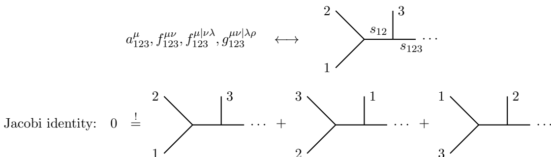
Figure 11. Diagrammatic interpretation of three-particle polarizations a_{123}^\mu, f_{123}^{\mu\nu}, f_{123}^{\mu|\nu\lambda} , and g_{123}^{\mu\nu|\lambda\rho} subject to kinematic Jacobi relations such as a_{123}^\mu + \text{cyc}(1, 2, 3) = 0 .
