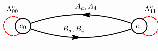
Figure 1. The \mathbb{C}^2/\mathbb{Z}_2(1, 1, 1, 1) quiver. The index a takes the values a = 1, 2, 3 . There are three adjoint fermi multiplets \Lambda^a at each nodes, and two sets of four chiral multiplets, A_i = (A_a, A_4) and B_i = (B_a, B_4) , in bifundamental representations. The quiver arrows have multiplicities equal to the number of distinct chiral or fermi multiplets.
