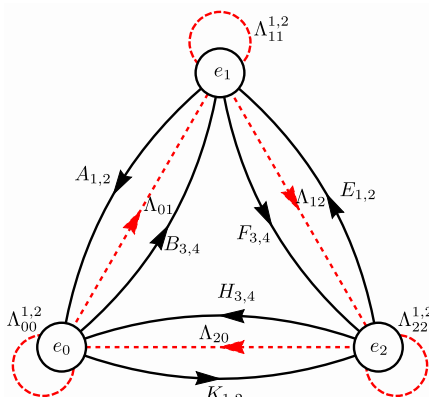
Figure 2. The \mathbb{C}^3/\mathbb{Z}_3(1,1,2,2) supersymmetric quiver, with all the chiral and fermi multiplets indicated explicitly.
