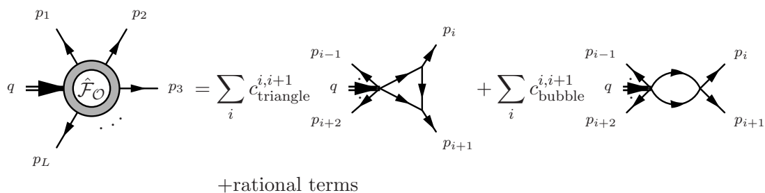
Figure 4. The one-loop correction to the form factor \hat{\mathcal{F}}_O for a minimal number of external fields can be written as a linear combination of one-mass triangle integrals, bubble integrals and rational terms. Here, the coefficients are labelled by the two momenta that leave the integrals on the right.
