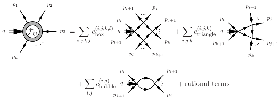
Figure 3. The one-loop correction to the colour-ordered form factor \hat{\mathcal{F}}_{\mathcal{O}} can be written as a linear combination of box integrals, triangle integrals, bubble integrals and rational terms. The coefficients are labelled by the different combinations of momenta flowing out of the corners of the integrals. While the on-shell momenta p_i are colour ordered, the off-shell momentum q of the operator does not take part in the colour ordering as the operator is a colour singlet.
