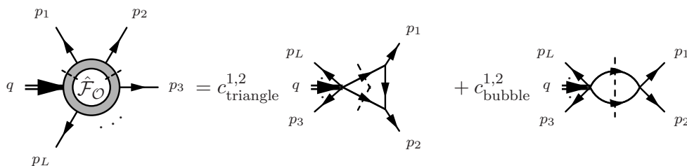
Figure 6. The double cut between p_1 , p_2 and the rest of the diagram isolates the triangle integral and bubble integral with external on-shell legs p_1 and p_2 . To obtain the bubble coefficient c_{\text{bubble}}^{1,2} , we bring the cut triangle integral and its known coefficient c_{\text{triangle}}^{1,2} to the l.h.s. of the equation. We then integrate on both sides of the equation over all components of the loop momentum that are not fixed by the cut.
