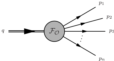
Figure 1. The momentum-space form factor of an operator \mathcal{O} . The operator has momentum q and is depicted as double line while the n on-shell fields with momenta p_i ( i = 1, \dots, n ) are depicted as single lines. The arrows indicate the direction of momentum flow.
