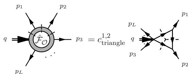
Figure 5. The triple cut between p_1 , p_2 and the rest of the diagram isolates the triangle integral with external on-shell legs p_1 and p_2 . To obtain its coefficient c_{\text{triangle}}^{1,2} , we integrate on both sides of the equation over all components of the loop momentum that are not fixed by the cut.
