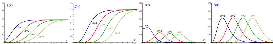
Figure 12. Profiles of the radially symmetric \phi -vortices for several values of the vorticity n in case C ( b_1 = 0, b_0 = c_0 = c_1 = 1 ) for the parameters \rho = a = e = 1 : from left to right the function f(r) , the function \beta(r) , the energy density \epsilon(r) and the magnetic field B(r) .
